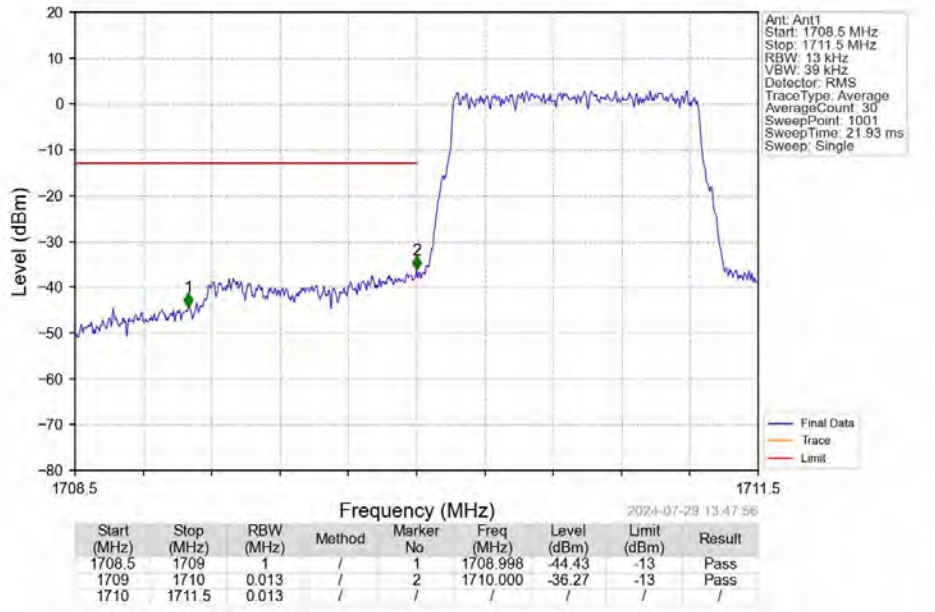
Band66_1.4MHz_QPSK_LCH_1710.7MHz_RB_6_0_NTNV
