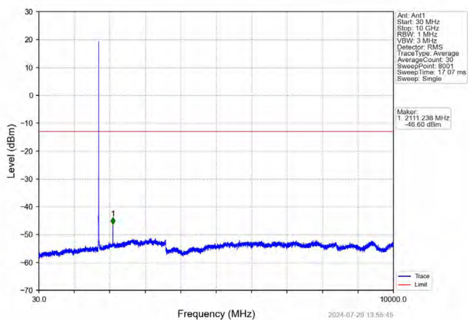
Band66_3MHz_16QAM_LCH_1711.5MHz_RB_1_0_NTNV
