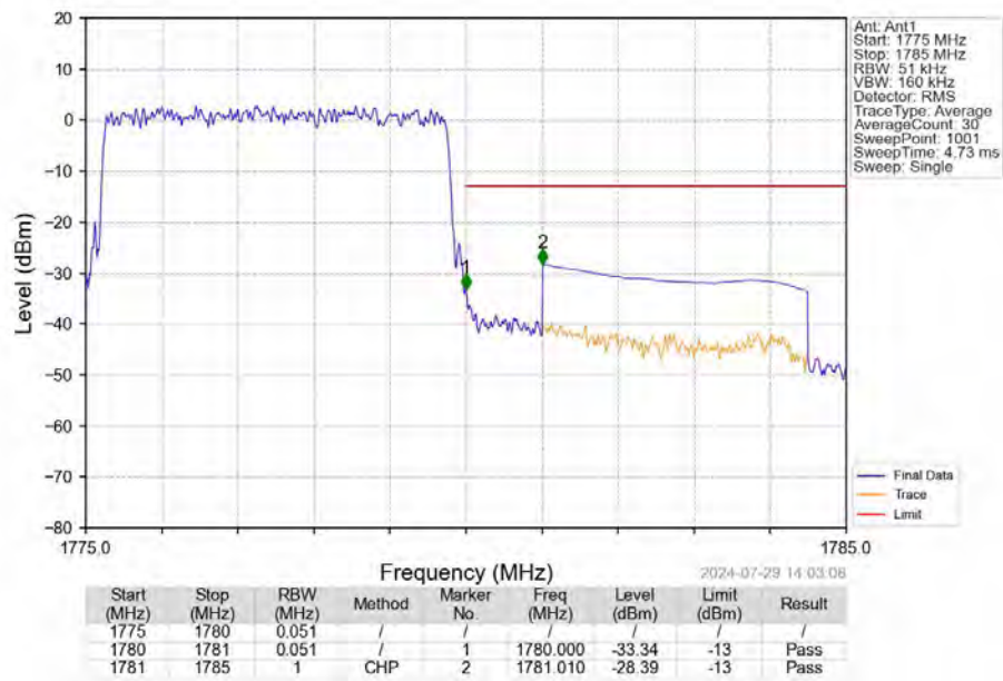
Band66_5MHz_QPSK_HCH_1777.5MHz_RB_25_0_NTNV
