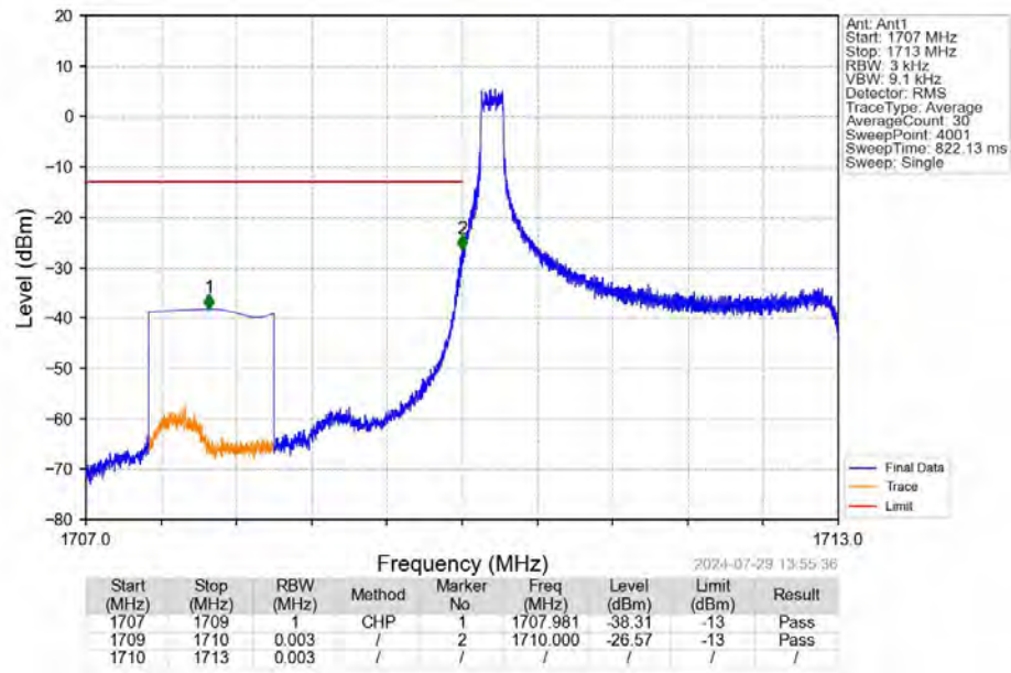
Band66_3MHz_16QAM_LCH_1711.5MHz_RB_1_0_NTNV
