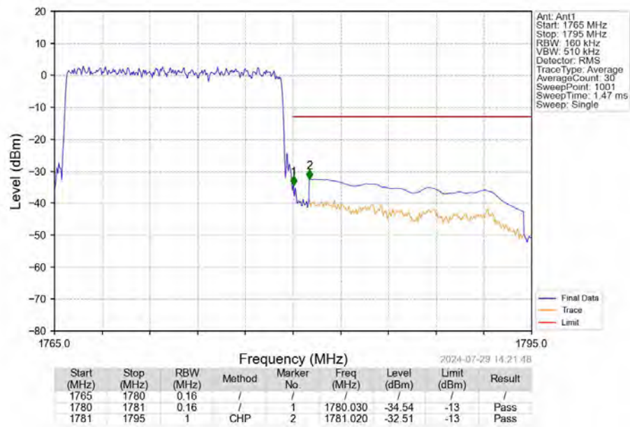
Band66_15MHz_QPSK_HCH_1772.5MHz_RB_75_0_NTNV
