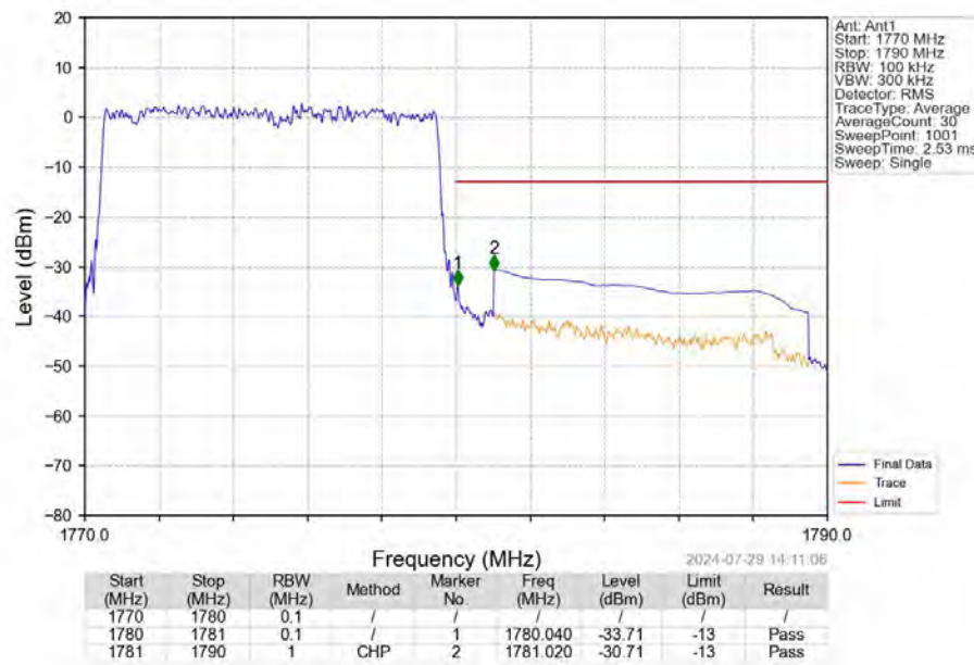
Band66_10MHz_QPSK_HCH_1775MHz_RB_50_0_NTNV
