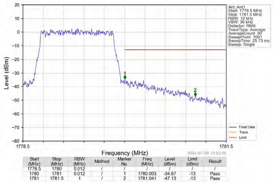
Band66_1.4MHz_16QAM_HCH_1779.3MHz_RB_6_0_NTNV
