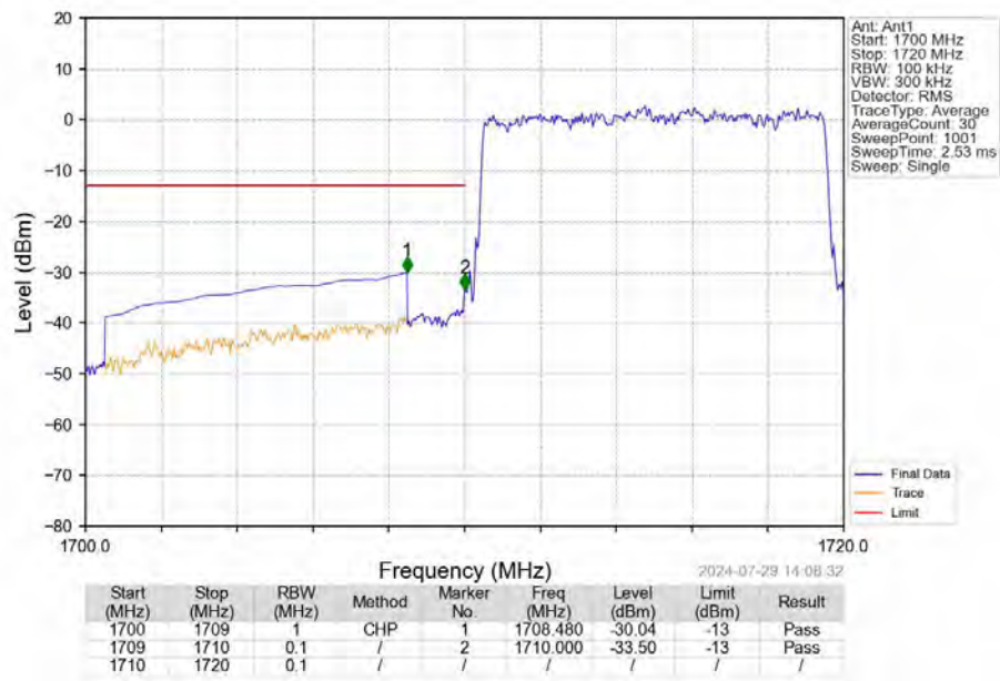
Band66_10MHz_16QAM_LCH_1715MHz_RB_50_0_NTNV
