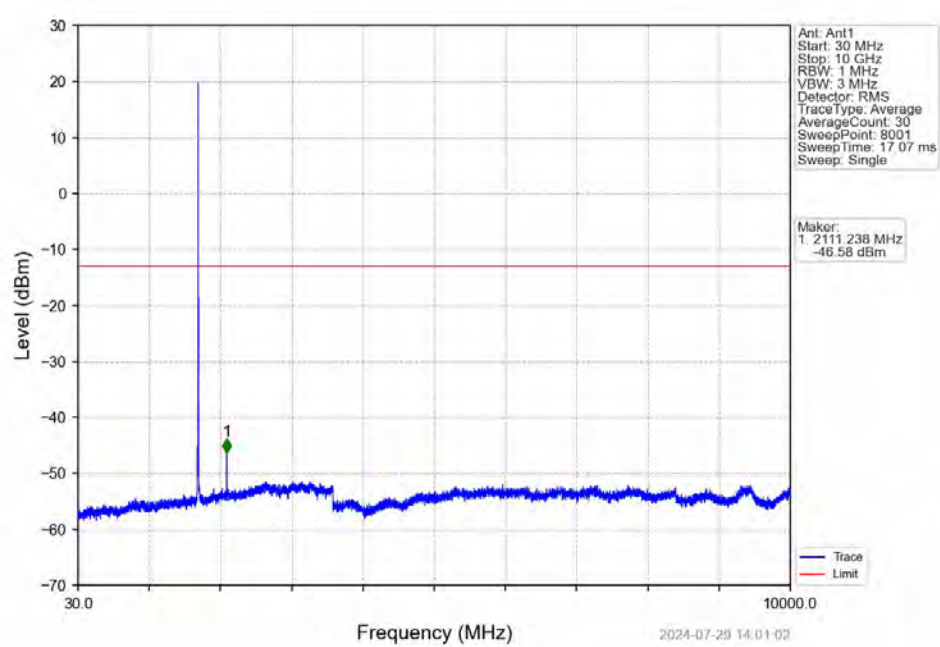
Band66_5MHz_16QAM_LCH_1712.5MHz_RB_1_0_NTNV
