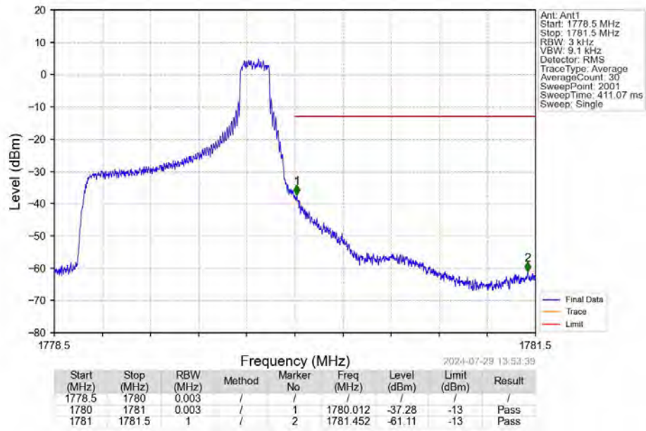
Band66_1.4MHz_16QAM_HCH_1779.3MHz_RB_1_5_NTNV
