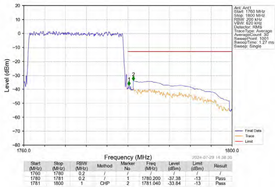
Band66_20MHz_16QAM_HCH_1770MHz_RB_100_0_NTNV
