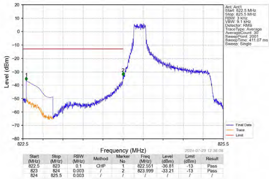
Band26b_1.4MHz_16QAM_LCH_824.7MHz_RB_1_0_NTNV
