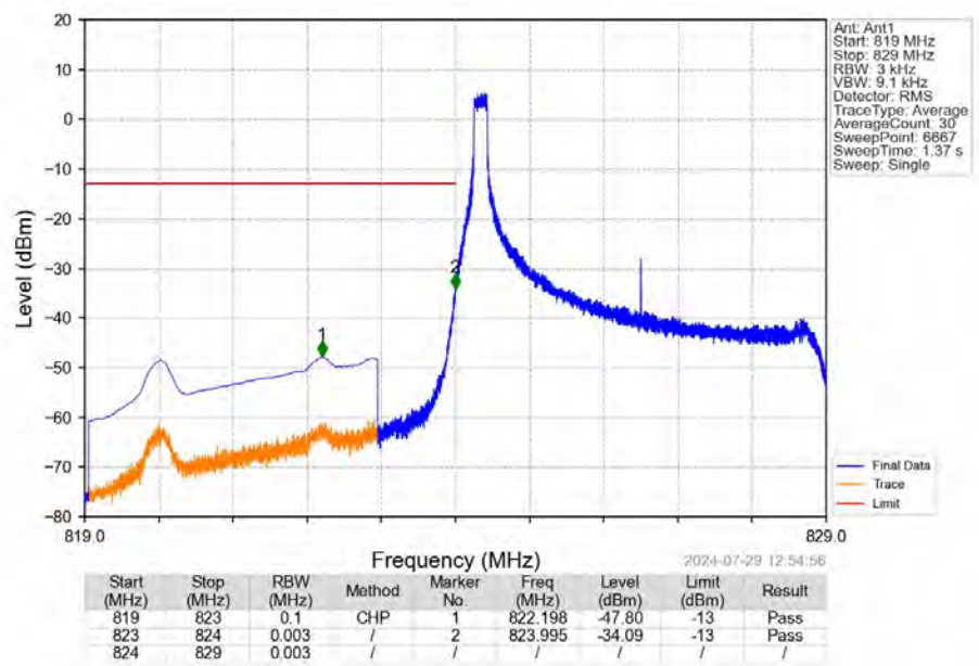
Band26b_5MHz_16QAM_LCH_826.5MHz_RB_1_0_NTNV
