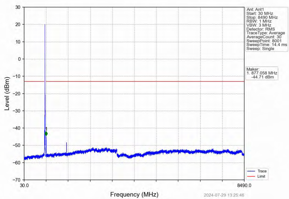
Band26b_15MHz_QPSK_MCH_836.5MHz_RB_1_0_NTNV
