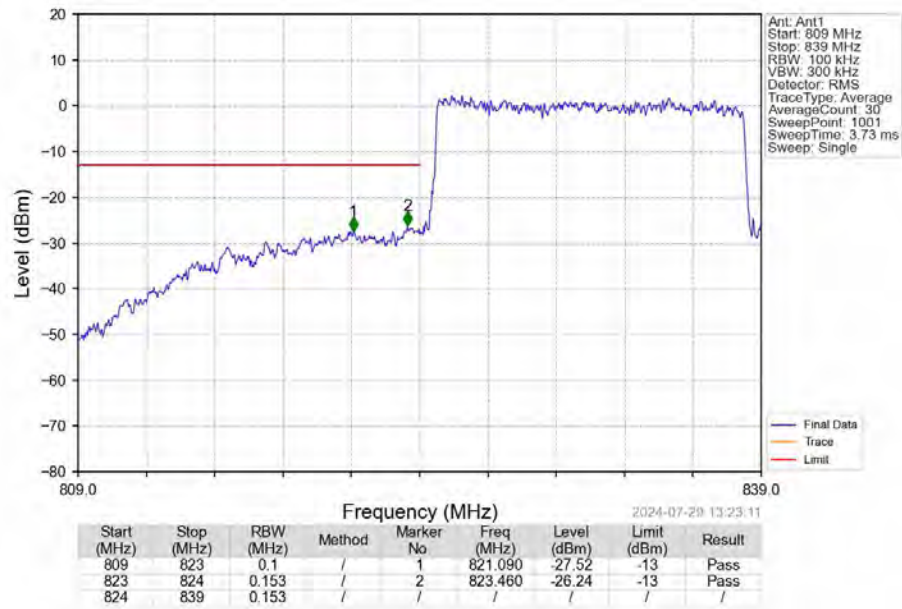
Band26b_15MHz_QPSK_LCH_831.5MHz_RB_75_0_NTNV
