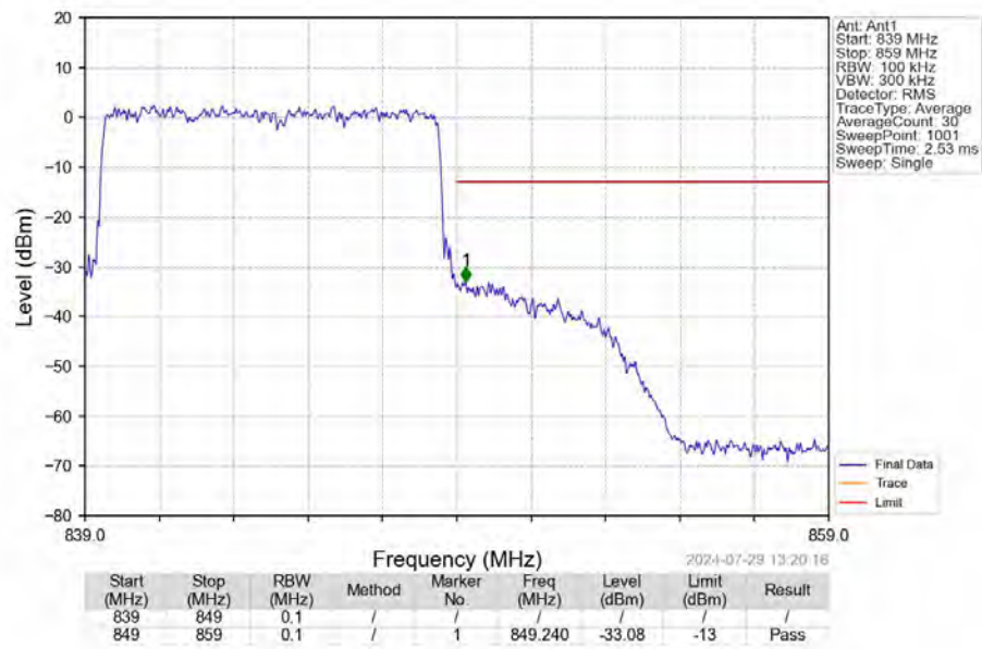
Band26b_10MHz_16QAM_HCH_844MHz_RB_50_0_NTNV
