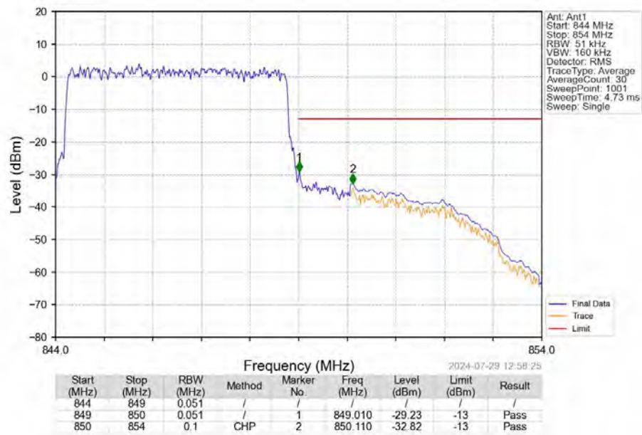
Band26b_5MHz_QPSK_HCH_846.5MHz_RB_25_0_NTNV
