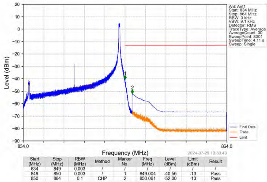
Band26b_15MHz_16QAM_HCH_841.5MHz_RB_1_74_NTNV
