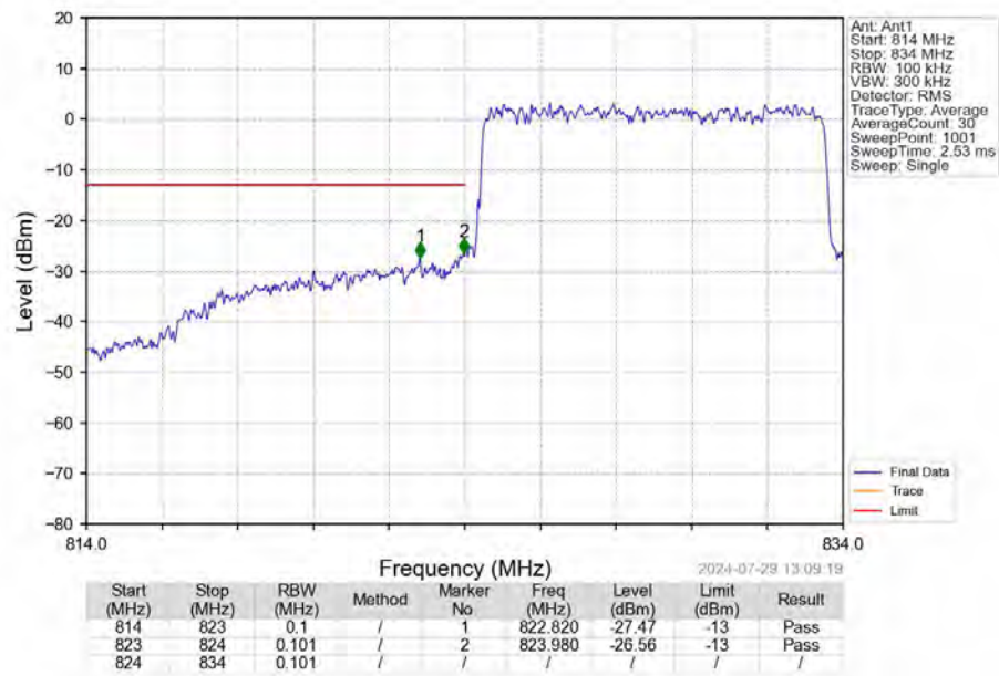
Band26b_10MHz_QPSK_LCH_829MHz_RB_50_0_NTNV
