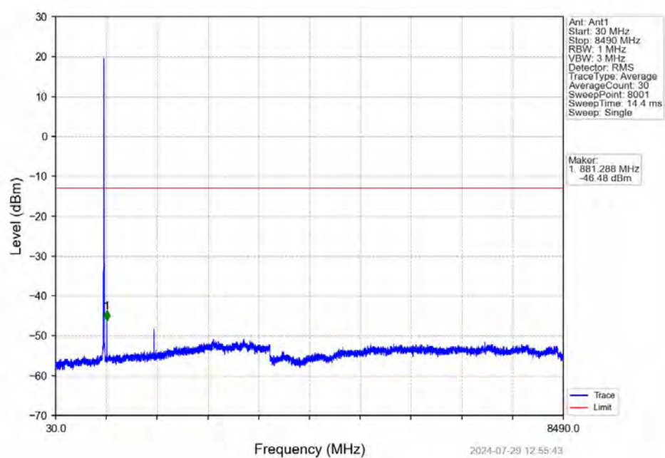
Band26b_5MHz_QPSK_MCH_836.5MHz_RB_1_0_NTNV
