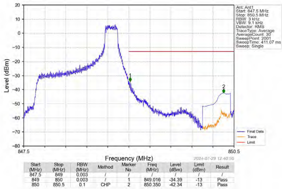
Band26b_1.4MHz_QPSK_HCH_848.3MHz_RB_1_5_NTNV
