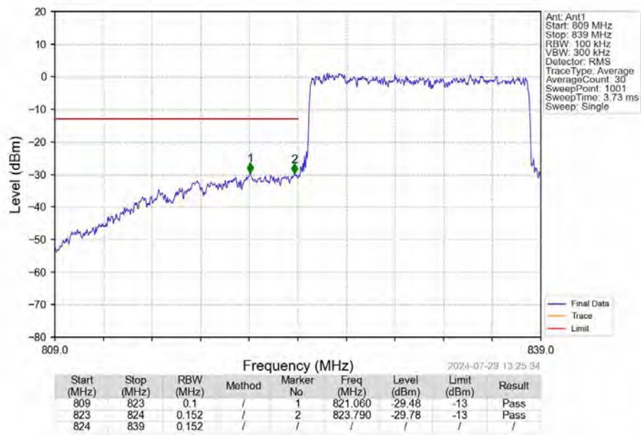
Band26b_15MHz_16QAM_LCH_831.5MHz_RB_75_0_NTNV
