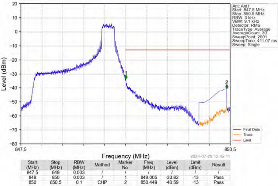
Band26b_1.4MHz_16QAM_HCH_848.3MHz_RB_1_5_NTNV
