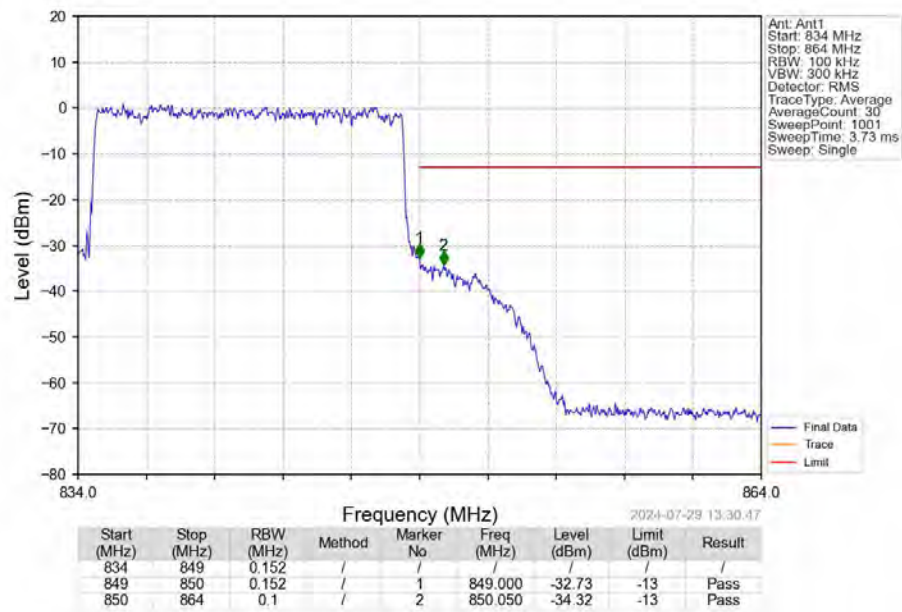
Band26b_15MHz_16QAM_HCH_841.5MHz_RB_75_0_NTNV
