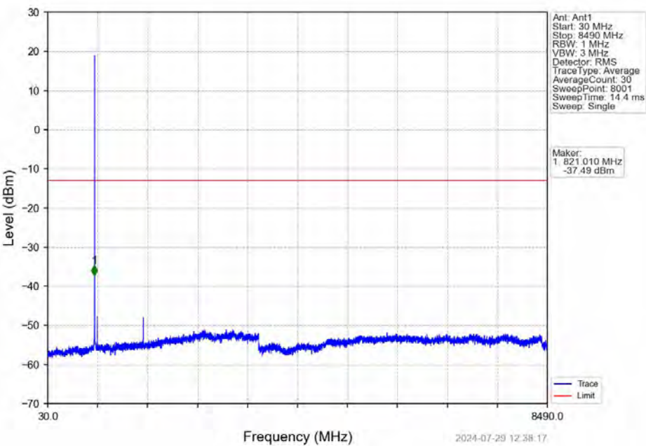
Band26b_1.4MHz_16QAM_LCH_824.7MHz_RB_6_0_NTNV
