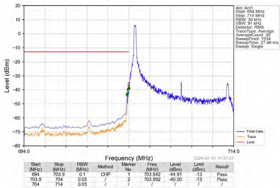
Band17_10MHz_16QAM_LCH_709MHz_RB_1_0_NTNV
