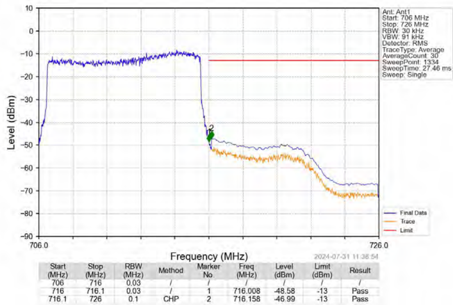
Band17_10MHz_16QAM_HCH_711MHz_RB_50_0_NTNV
