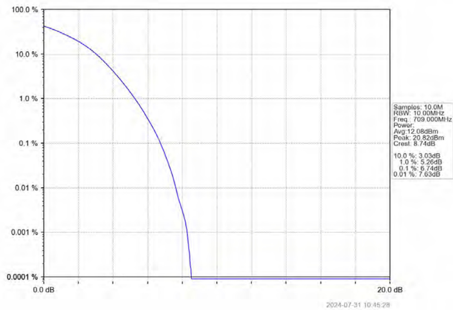
Band17_10MHz_16QAM_LCH_709MHz_RB_50_0_NTNV
