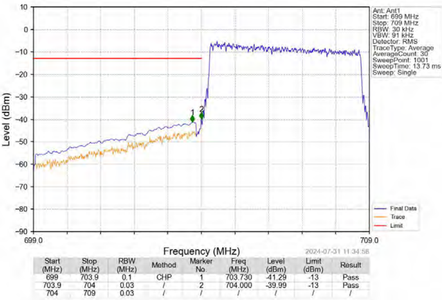
Band17_5MHz_QPSK_LCH_706.5MHz_RB_25_0_NTNV
