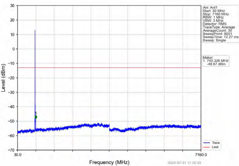
Band17_5MHz_QPSK_MCH_710MHz_RB_1_0_NTNV
