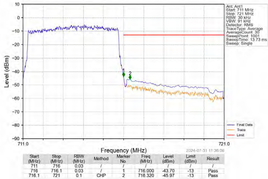
Band17_5MHz_QPSK_HCH_713.5MHz_RB_25_0_NTNV
