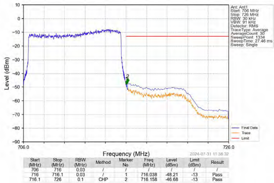
Band17_10MHz_QPSK_HCH_711MHz_RB_50_0_NTNV
