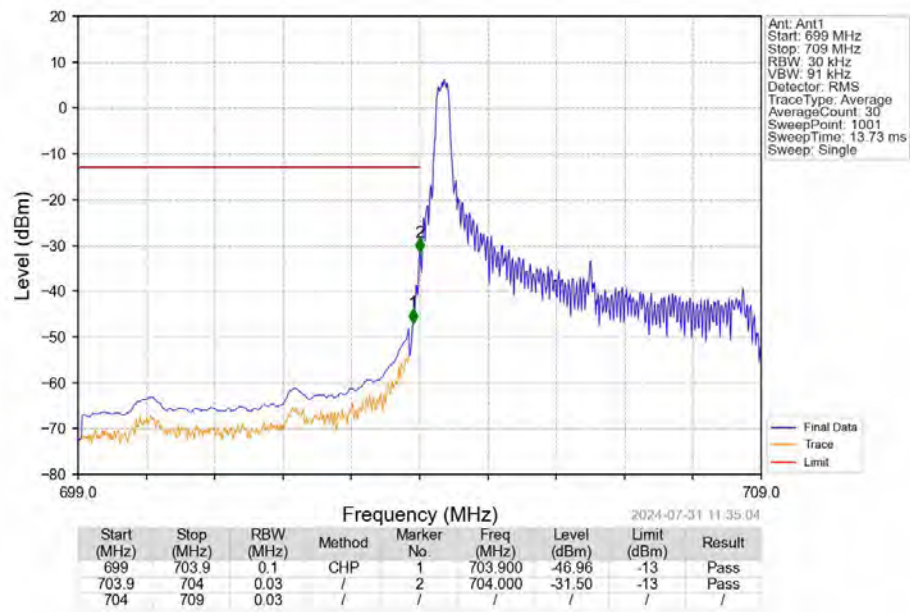
Band17_5MHz_16QAM_LCH_706.5MHz_RB_1_0_NTNV
