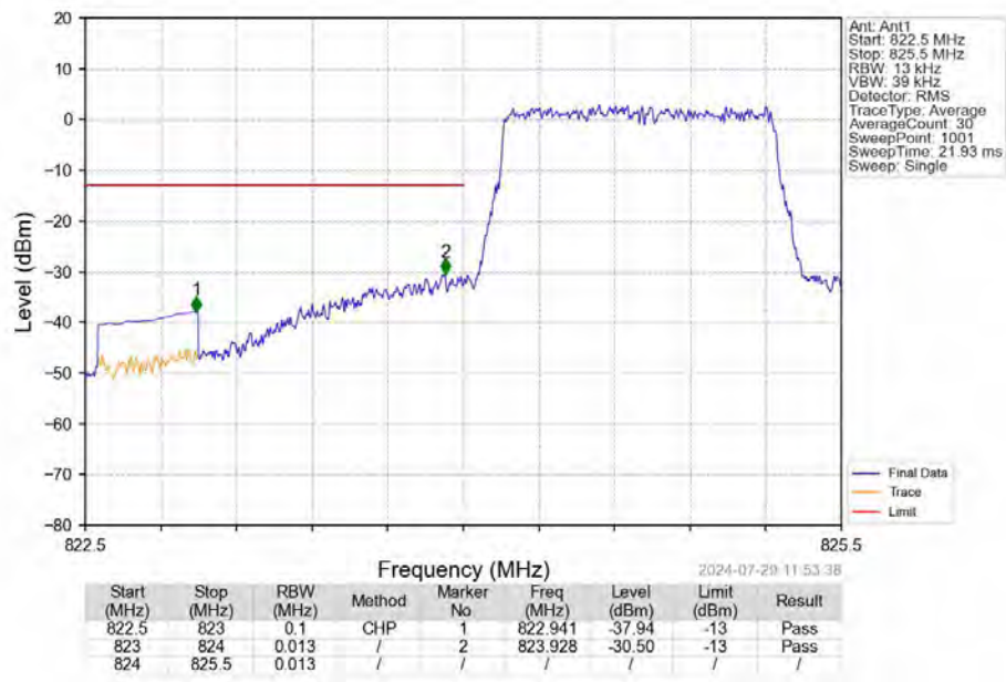
Band5_1.4MHz_16QAM_LCH_824.7MHz_RB_6_0_NTNV
