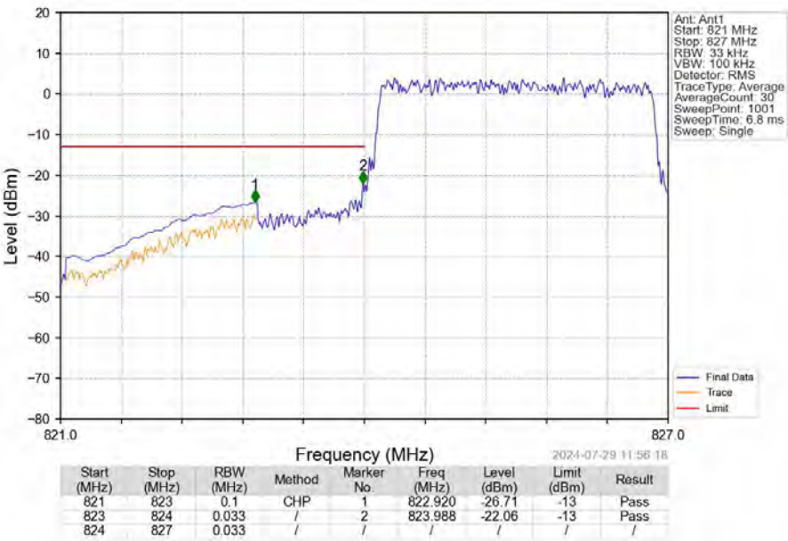
Band5_3MHz_QPSK_LCH_825.5MHz_RB_15_0_NTNV
