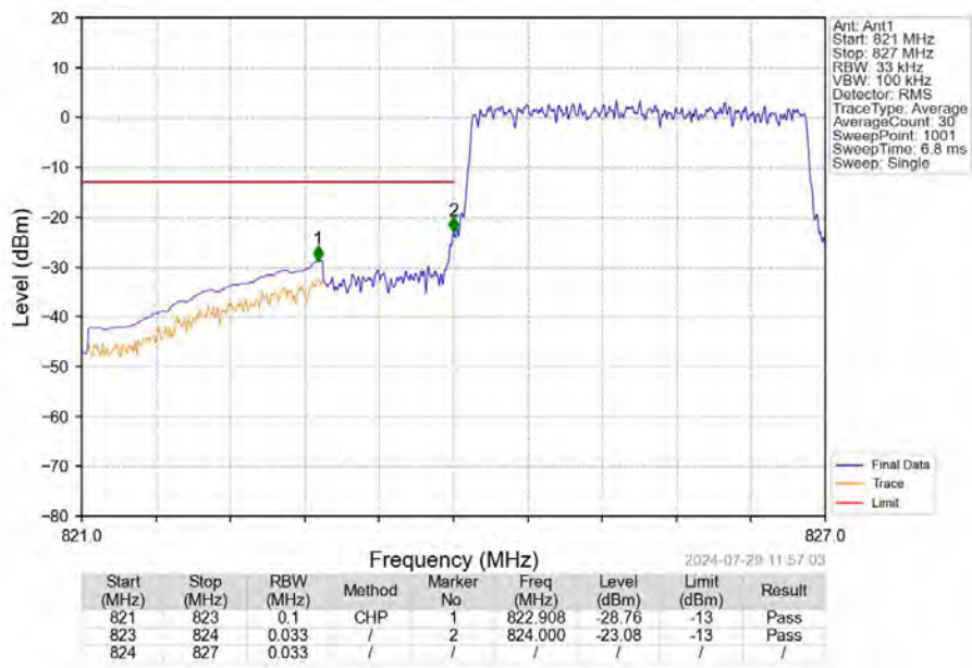
Band5_3MHz_16QAM_LCH_825.5MHz_RB_15_0_NTNV
