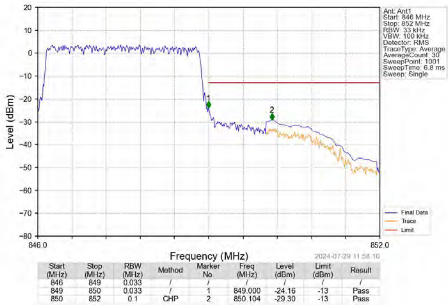
Band5_3MHz_QPSK_HCH_847.5MHz_RB_15_0_NTNV
