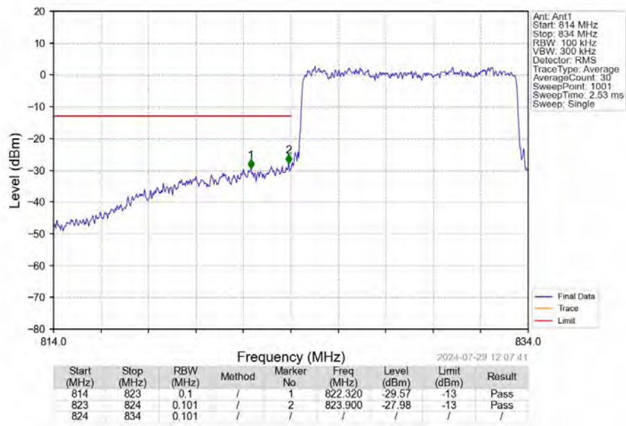
Band5_10MHz_16QAM_LCH_829MHz_RB_50_0_NTNV
