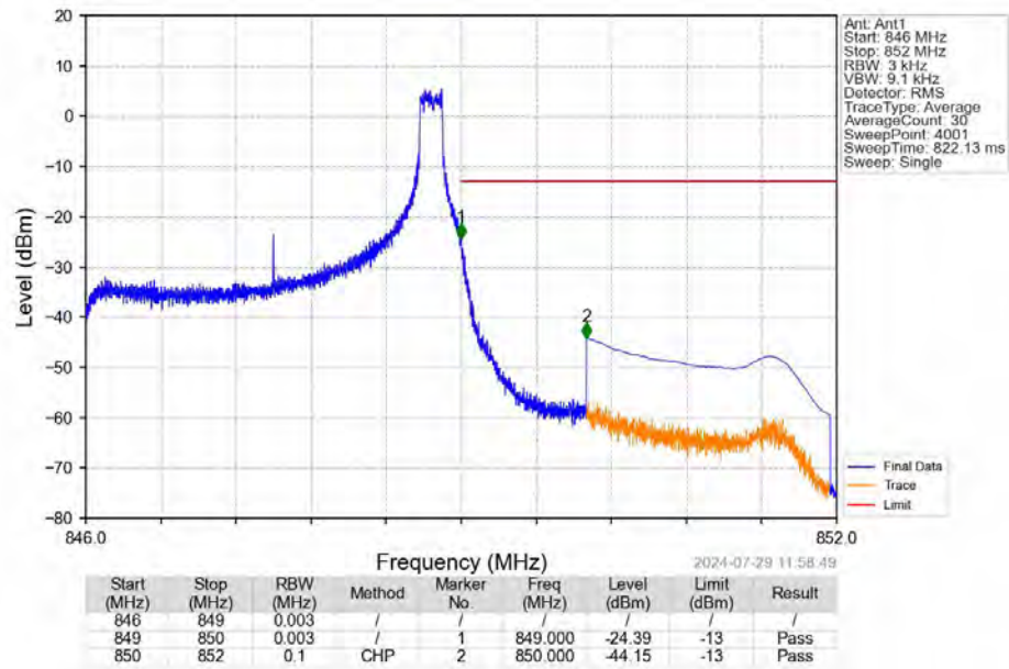
Band5_3MHz_16QAM_HCH_847.5MHz_RB_1_14_NTNV
