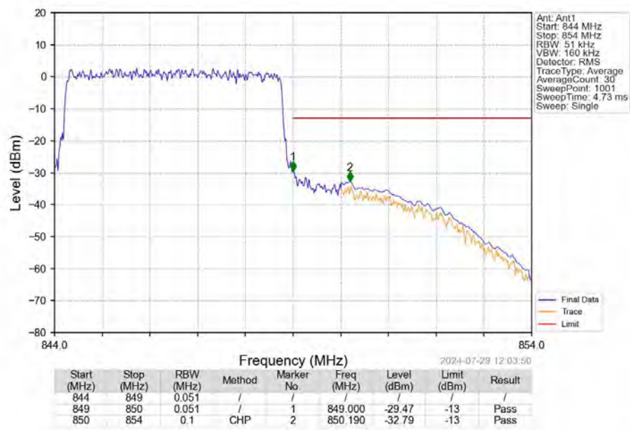
Band5_5MHz_16QAM_HCH_846.5MHz_RB_25_0_NTNV
