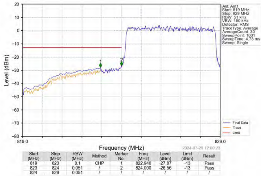
Band5_5MHz_QPSK_LCH_826.5MHz_RB_25_0_NTNV
