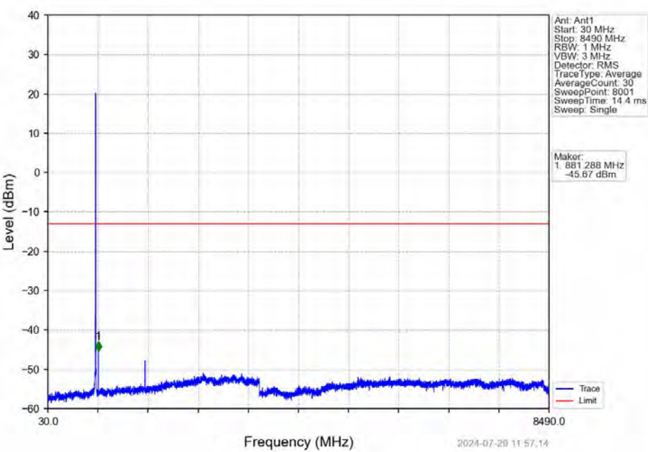
Band5_3MHz_QPSK_MCH_836.5MHz_RB_1_0_NTNV
