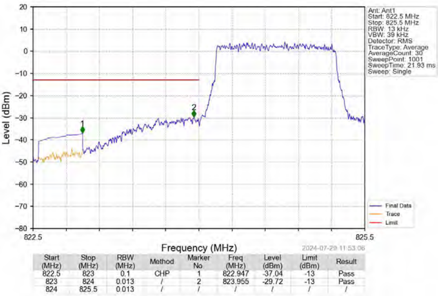
Band5_1.4MHz_QPSK_LCH_824.7MHz_RB_6_0_NTNV
