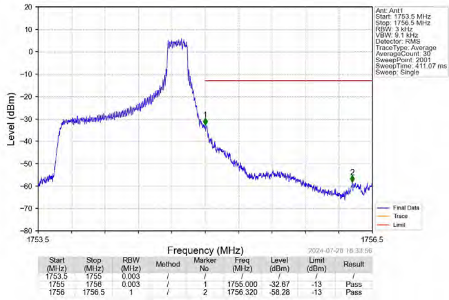
Band4_1.4MHz_QPSK_HCH_1754.3MHz_RB_1_5_NTNV
