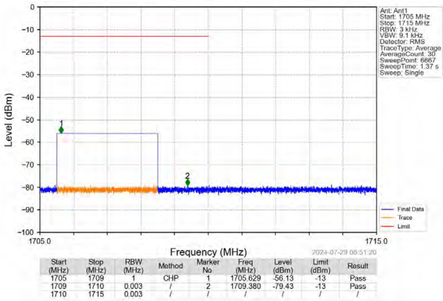
Band4_5MHz_16QAM_LCH_1712.5MHz_RB_1_0_NTNV
