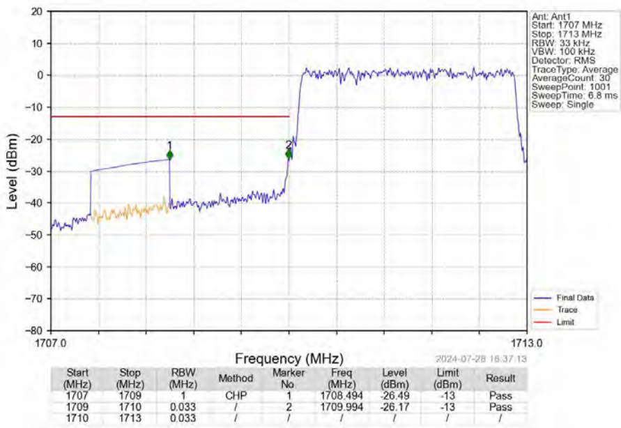
Band4_3MHz_16QAM_LCH_1711.5MHz_RB_15_0_NTNV
