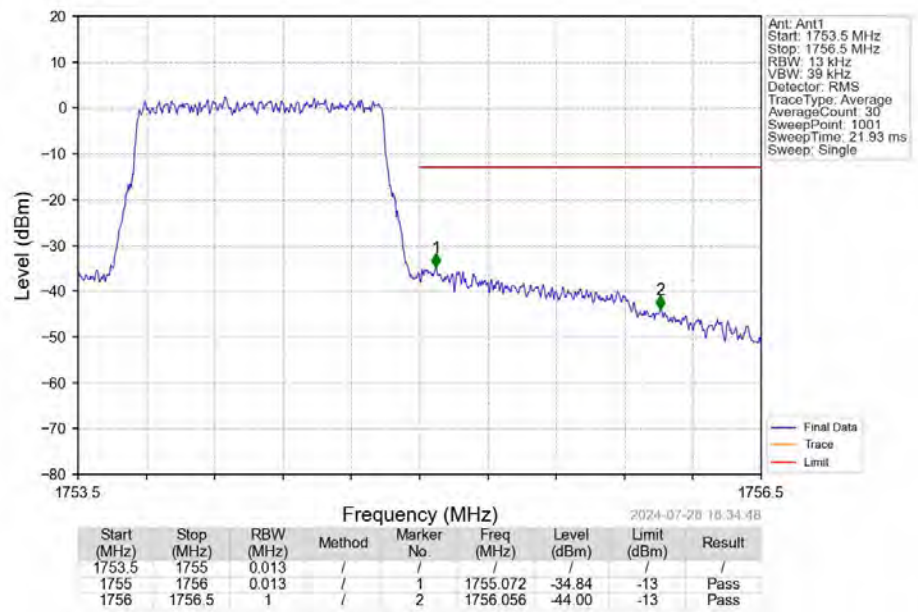
Band4_1.4MHz_16QAM_HCH_1754.3MHz_RB_6_0_NTNV
