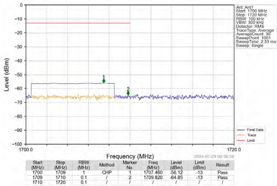
Band4_10MHz_QPSK_LCH_1715MHz_RB_50_0_NTNV
