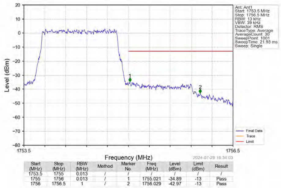
Band4_1.4MHz_QPSK_HCH_1754.3MHz_RB_6_0_NTNV
