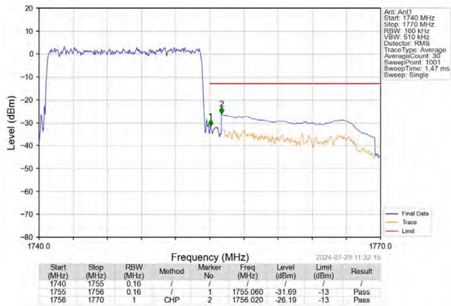
Band4_15MHz_QPSK_HCH_1747.5MHz_RB_75_0_NTNV
