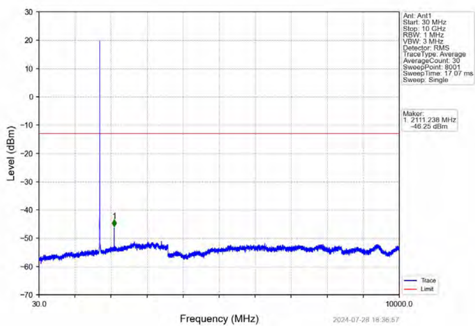
Band4_3MHz_16QAM_LCH_1711.5MHz_RB_1_0_NTNV
