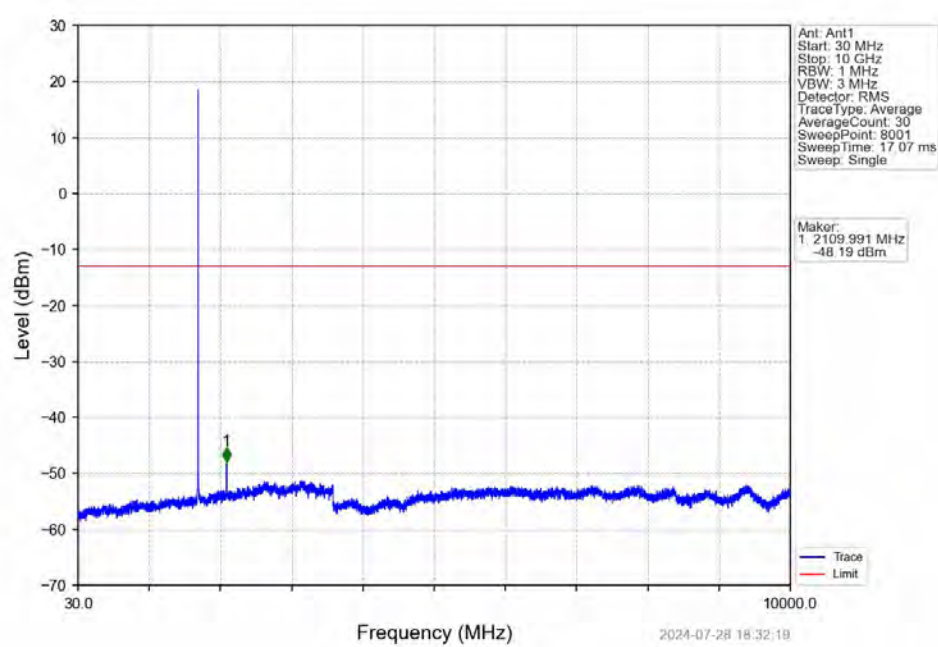
Band4_1.4MHz_16QAM_LCH_1710.7MHz_RB_1_0_NTNV
