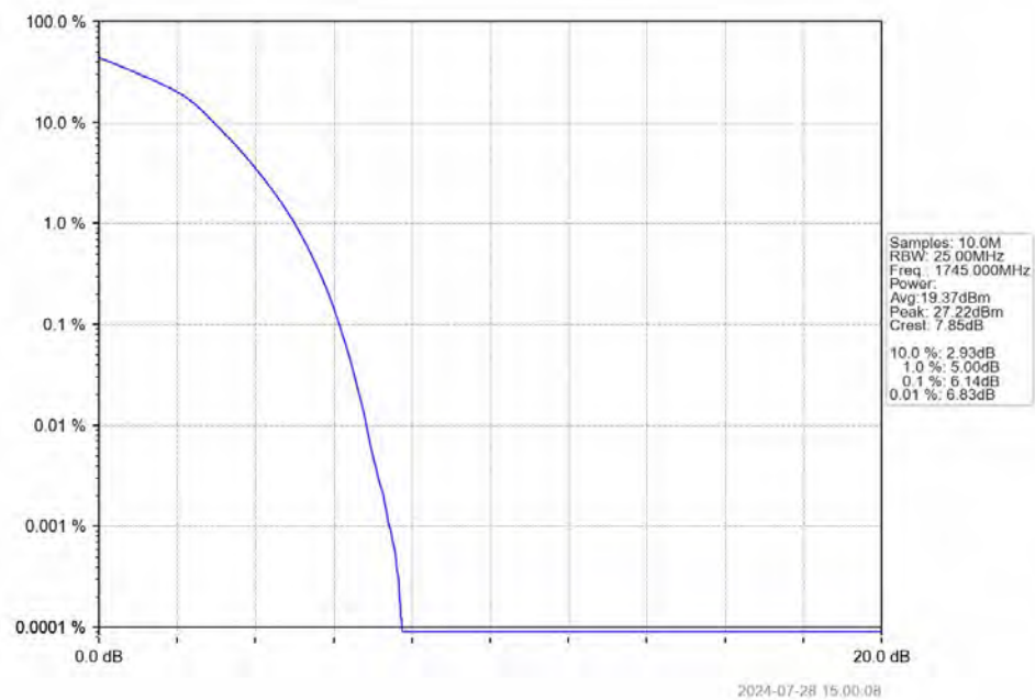
Band4_20MHz_16QAM_HCH_1745MHz_RB_100_0_NTNV
