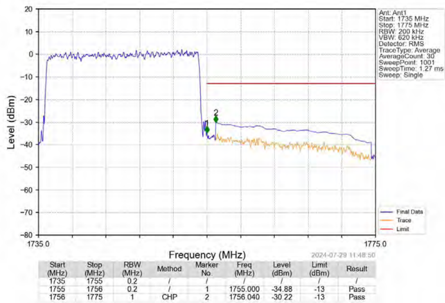
Band4_20MHz_16QAM_HCH_1745MHz_RB_100_0_NTNV
