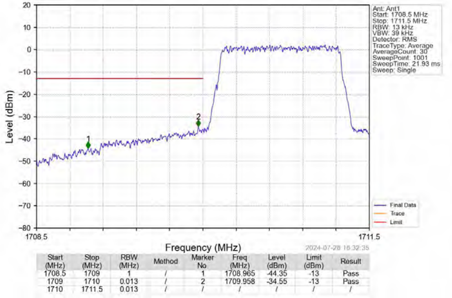
Band4_1.4MHz_16QAM_LCH_1710.7MHz_RB_6_0_NTNV
