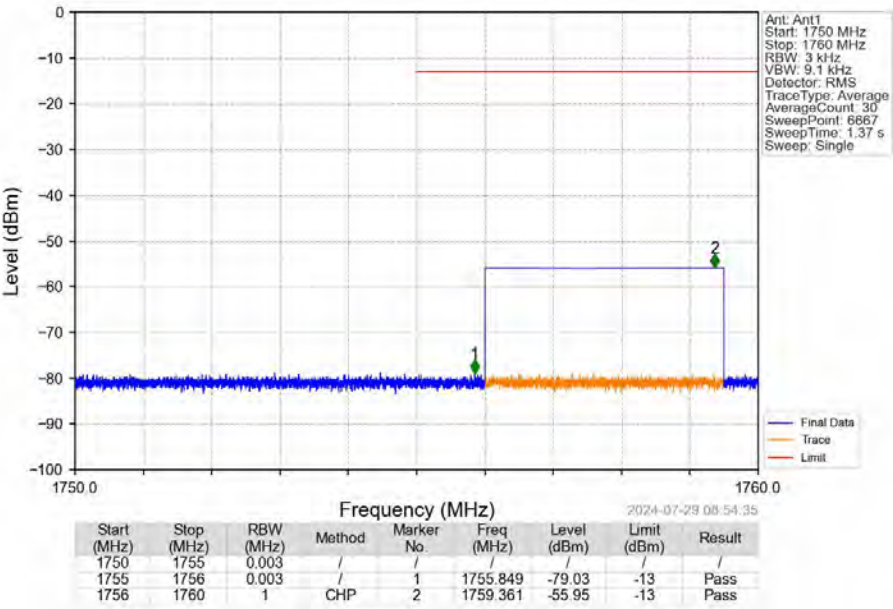
Band4_5MHz_16QAM_HCH_1752.5MHz_RB_1_24_NTNV
