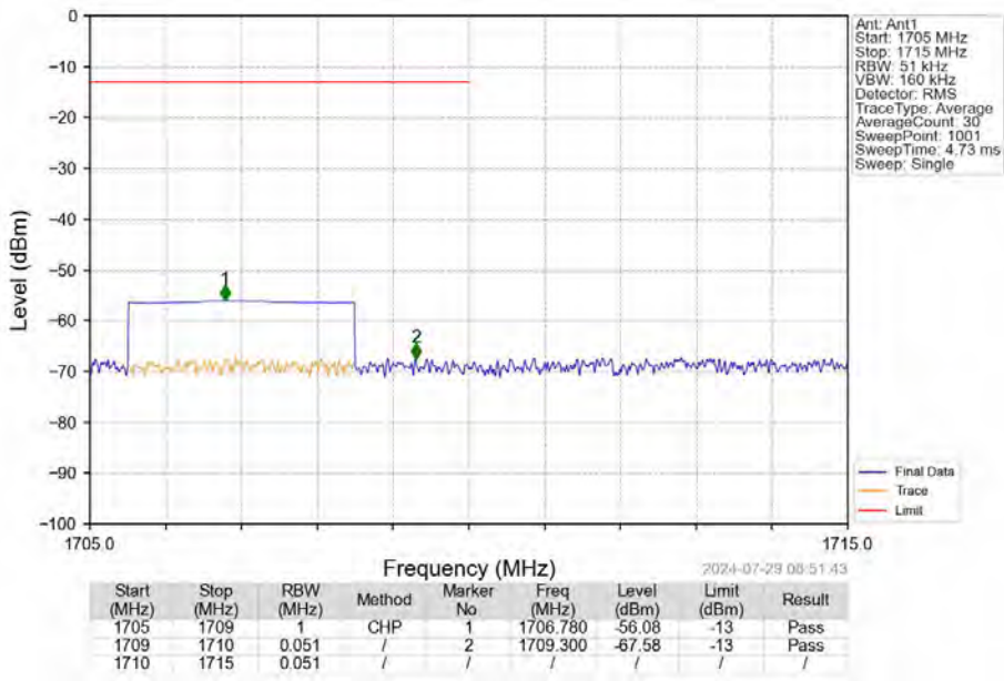
Band4_5MHz_16QAM_LCH_1712.5MHz_RB_25_0_NTNV
