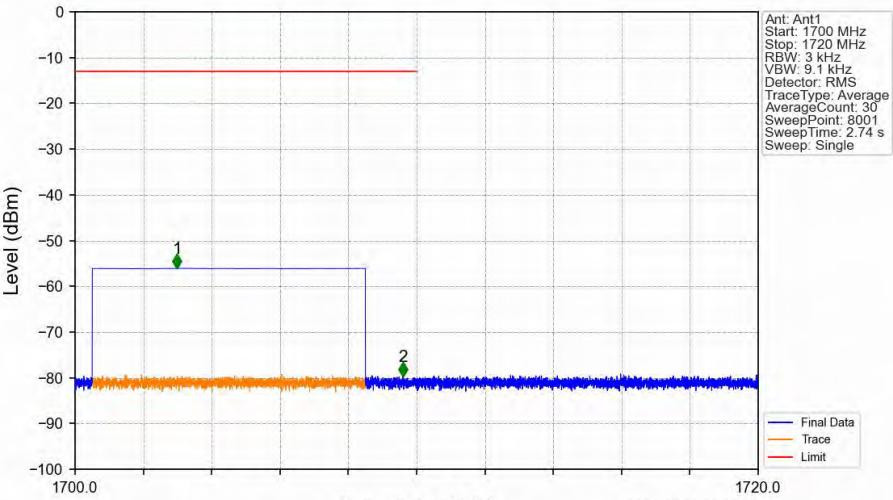
Band4_10MHz_16QAM_LCH_1715MHz_RB_1_0_NTNV
