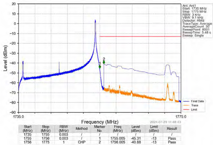
Band4_20MHz_16QAM_HCH_1745MHz_RB_1_99_NTNV
