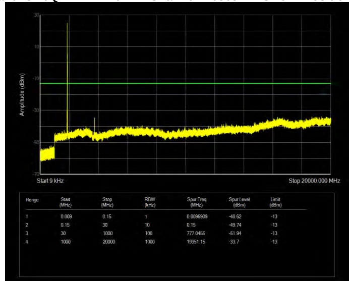
Band25 16QAM BW=10MHz Channel=26640 RB Size=1 Position=#0
