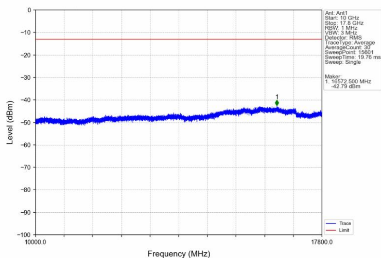
Band66 15MHz 16QAM HCH 1772.5MHz RB 1 0 NTNV
