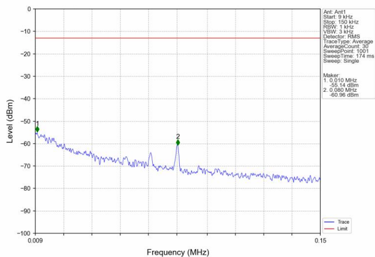
Band66 15MHz 16QAM HCH 1772.5MHz RB 1 0 NTNV
