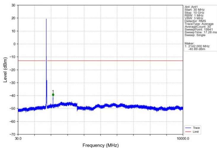
Band66 20MHz 16QAM MCH 1745MHz RB 1 0 NTV
