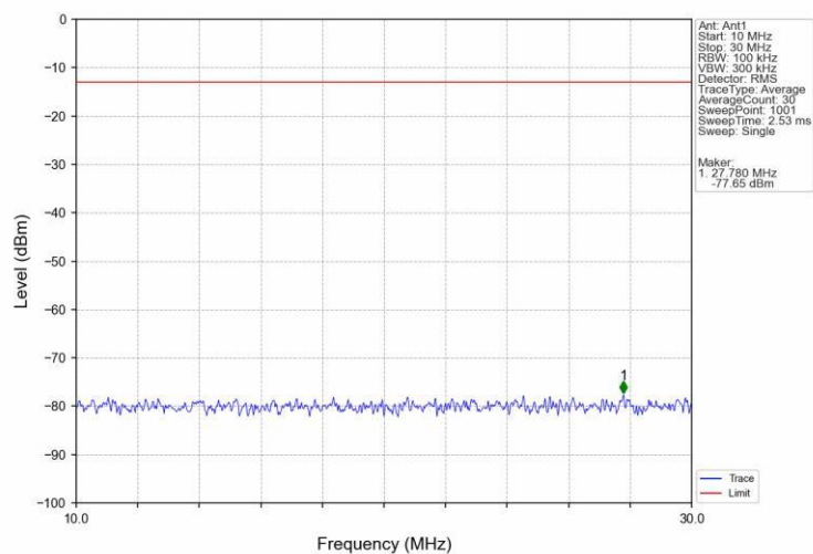
Band66 15MHz 16QAM HCH 1772.5MHz RB 1 0 NTN
