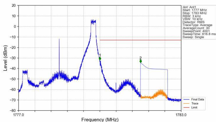
Band66 3MHz 16QAM HCH 1778.5MHz RB 1 14 NTN
