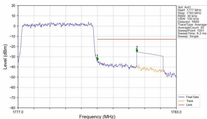
Band66 3MHz 16QAM HCH 1778.5MHz RB 15 0 NTN
