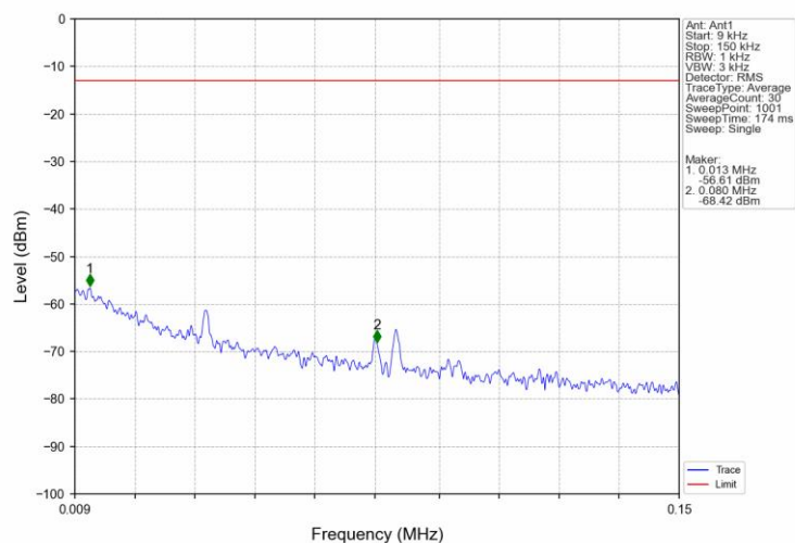
Band71 15MHz 16QAM HCH 690.5MHz RB 1 0 NTNV
