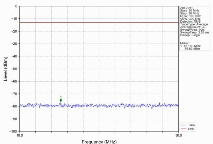
Band71_15MHz_16QAM_LCH_670.5MHz_RB_1_0_NTNV
