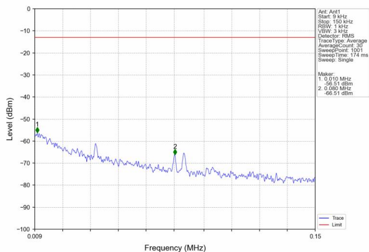
Band71 15MHz 16QAM MCH 680.5MHz RB 1 0 NTNV
