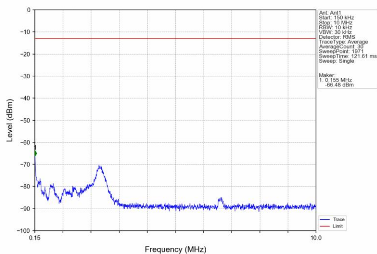
Band71_15MHz_QPSK_HCH_690.5MHz_RB_1_0_NTNV
