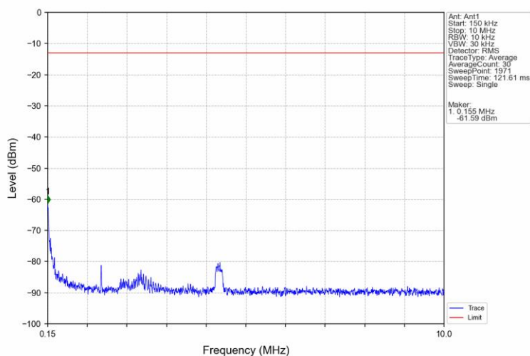
Band26a_10MHz_16QAM_LCH_819MHz_RB_1_0_NTNV
