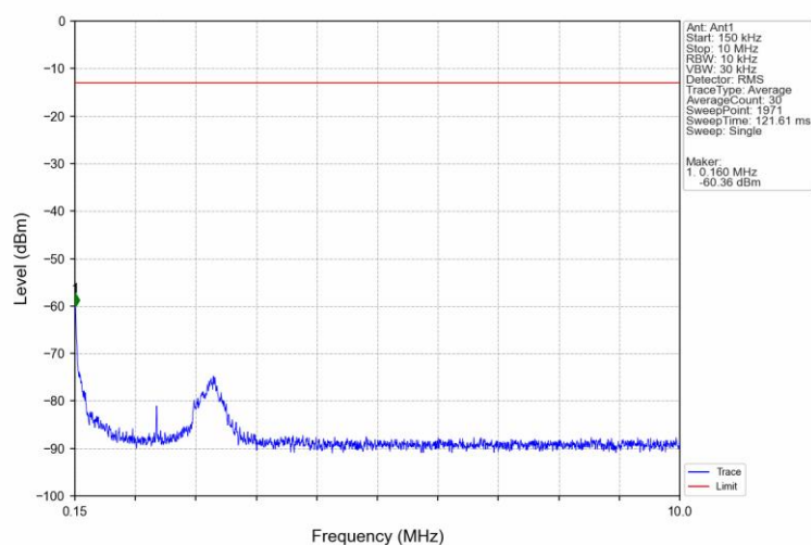
Band26a_5MHz_QPSK_LCH_816.5MHz_RB_1_0_NTNV
