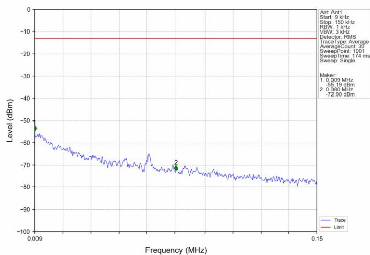
Band26a_5MHz_QPSK_LCH_816.5MHz_RB_1_0_NTNV
