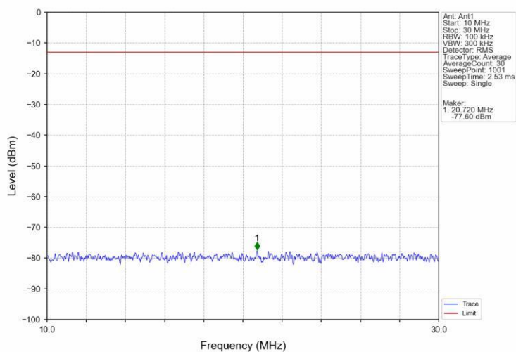
Band26a_10MHz_16QAM_LCH_819MHz_RB_1_0_NTNV
