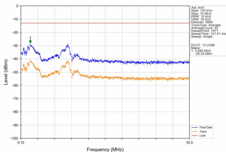
PCS1900 EGPRS MCH 1880MHz 1 TX Slot NTN
