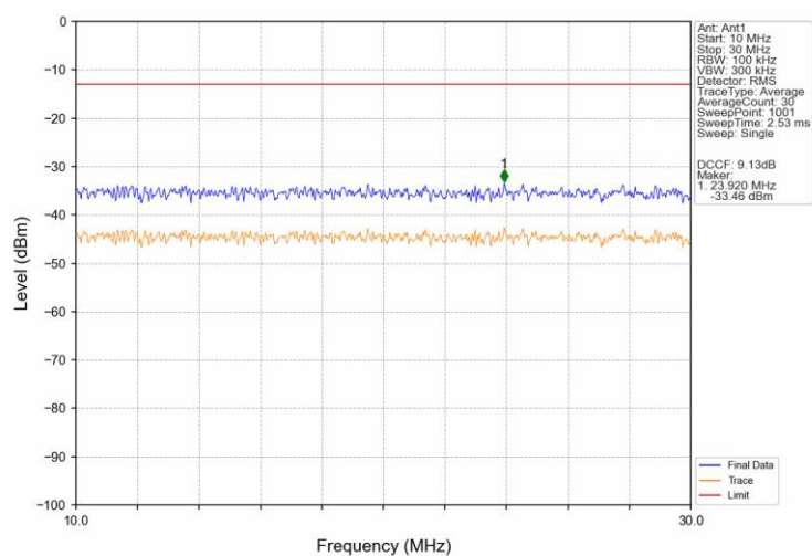
PCS1900 GPRS HCH 1909.8MHz 1 TX Slot NTN
