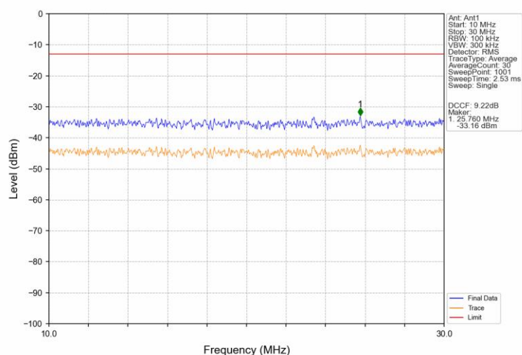
PCS1900 EGPRS HCH 1909.8MHz 1 TX Slot NTN
