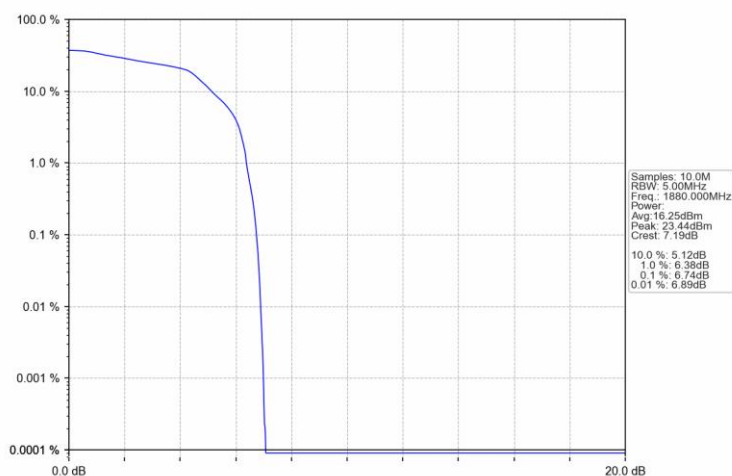
PCS1900 EGPRS MCH 1880MHz 4 TX Slots NTN
