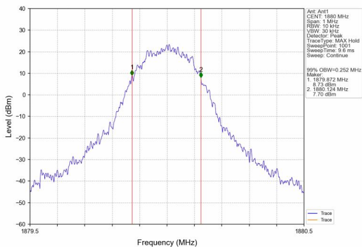
PCS1900 EGPRS MCH 1880MHz 1 TX Slot NTN
