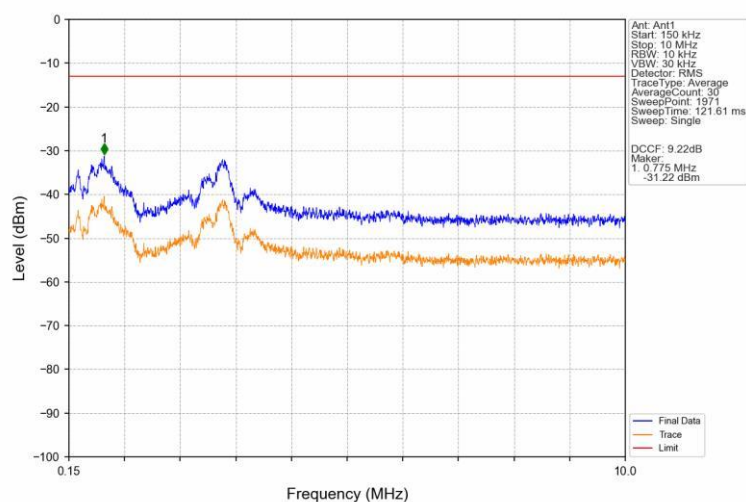
PCS1900 EGPRS LCH 1850.2MHz 1 TX Slot NTN
