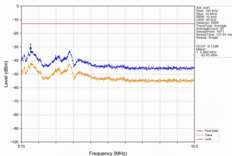
PCS1900 GPRS HCH 1909.8MHz 1 TX Slot NTN
