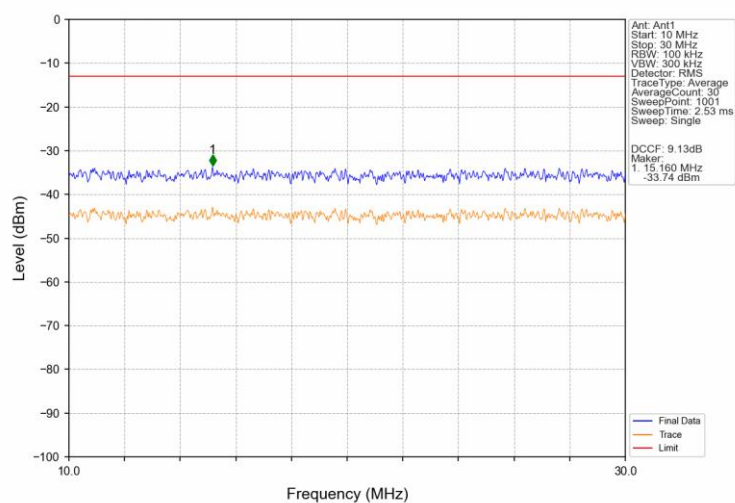
PCS1900_GPRS_LCH_1850.2MHz_1 TX Slot_NTNV
