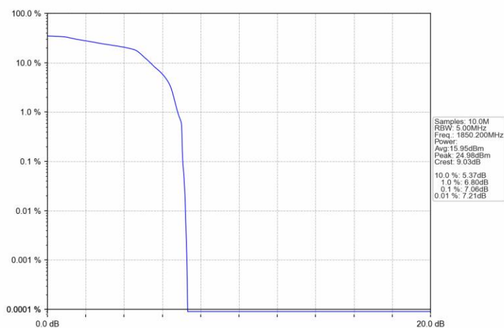
PCS1900 EGPRS LCH 1850.2MHz 4 TX Slots NTN
