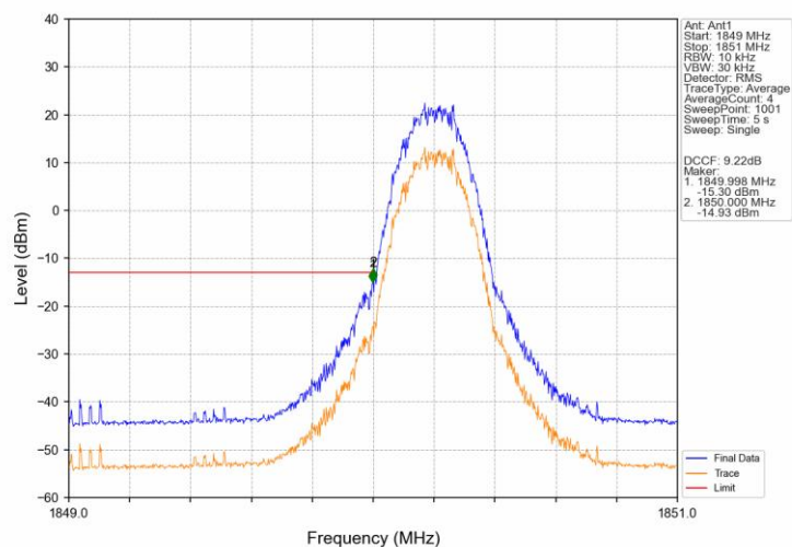
PCS1900 EGPRS LCH 1850.2MHz 1 TX Slot NTN
