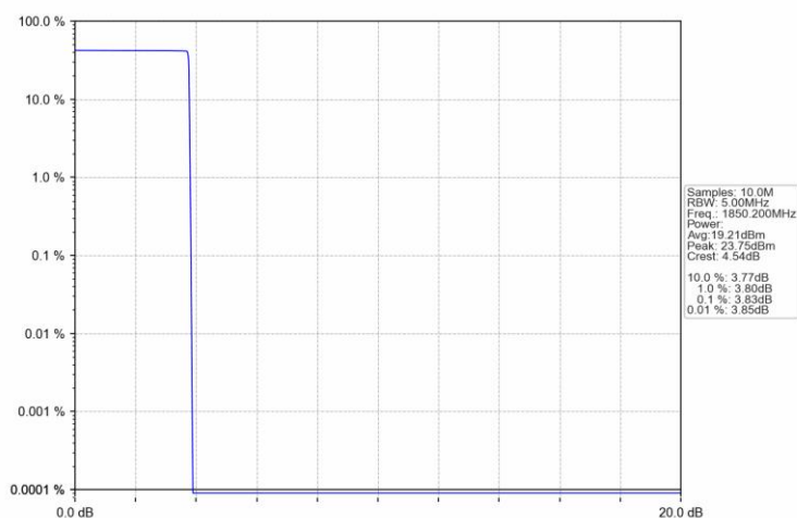
PCS1900 GPRS LCH 1850.2MHz_4 TX Slots NTN
