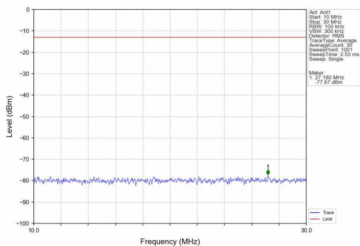
Band25 20MHz QPSK MCH 1882.5MHz RB 1 0 NTNV
