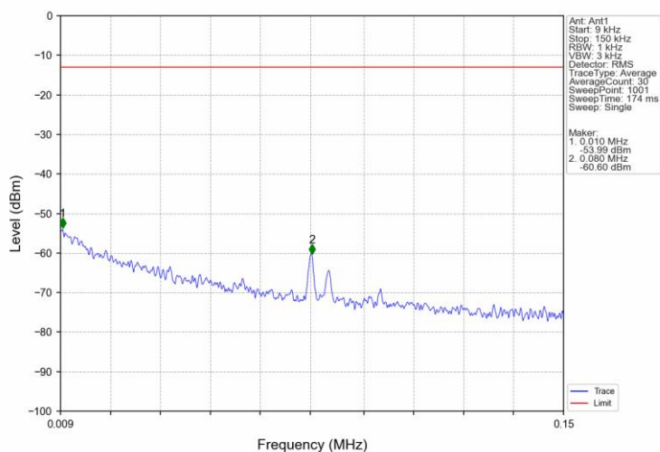
Band25 15MHz QPSK HCH 1907.5MHz RB 1 0 NTNV
