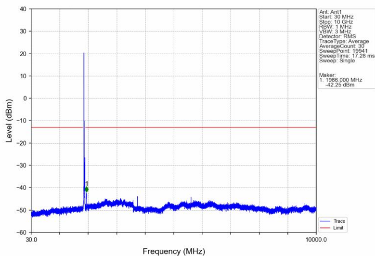
Band25 20MHz 16QAM MCH 1882.5MHz RB 1 0 NTN
