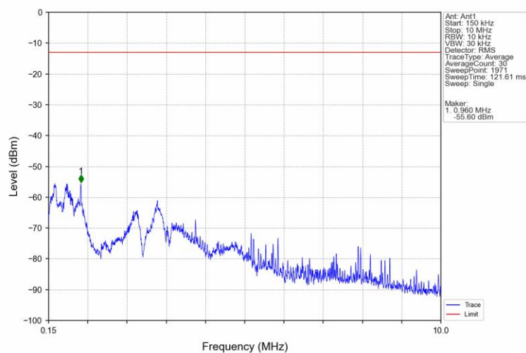
Band5_HSDPA_LCH_826.4MHz_Subtest 1_NTNV
