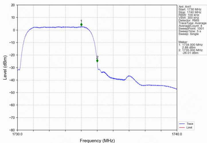
Band4_HSDPA_MCH_1732.6MHz_Subtest 1_NTNV
