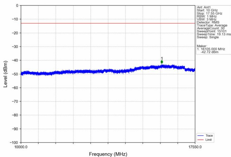
Band4 HSDPA MCH 1732.6MHz Subtest 1 NTNV
