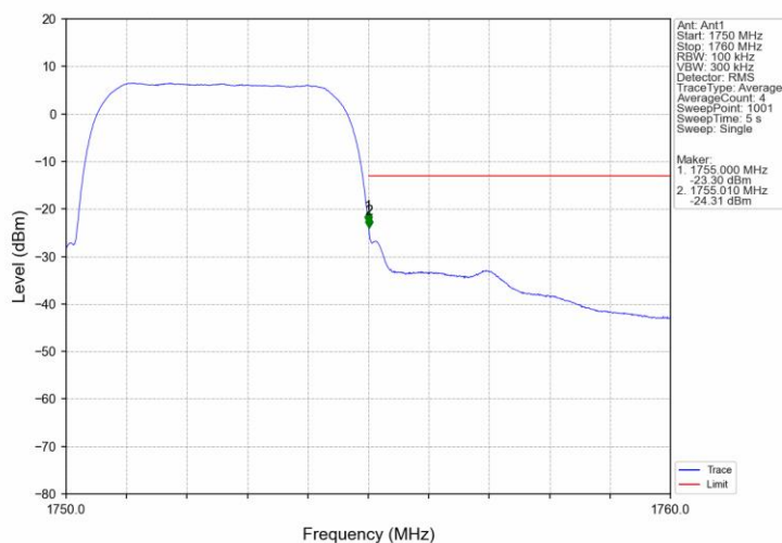
Band4_RMC_HCH_1752.6MHz_12.2kbps_RMC_NTNV
