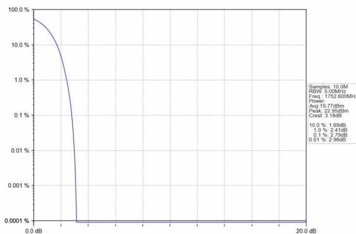
Band4_RMC_HCH_1752.6MHz_12.2kbps_RMC_NTNV
