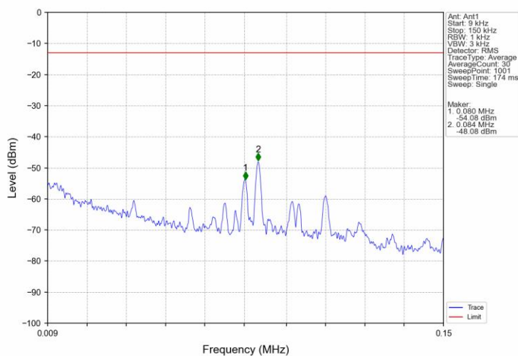
Band4 HSUPA HCH 1752.6MHz Subtest 1 NTNV
