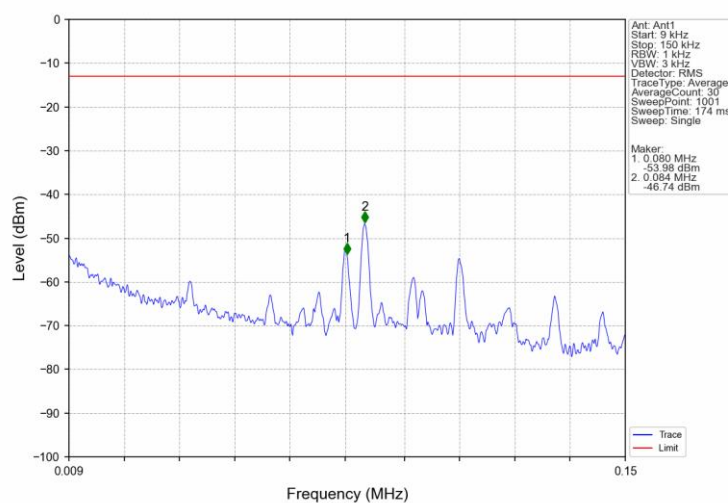
Band4_HSDPA_LCH_1712.4MHz_Subtest 1_NTNV
