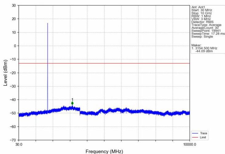
Band4_RMC_LCH_1712.4MHz_12.2kbps_RMC_NTNV
