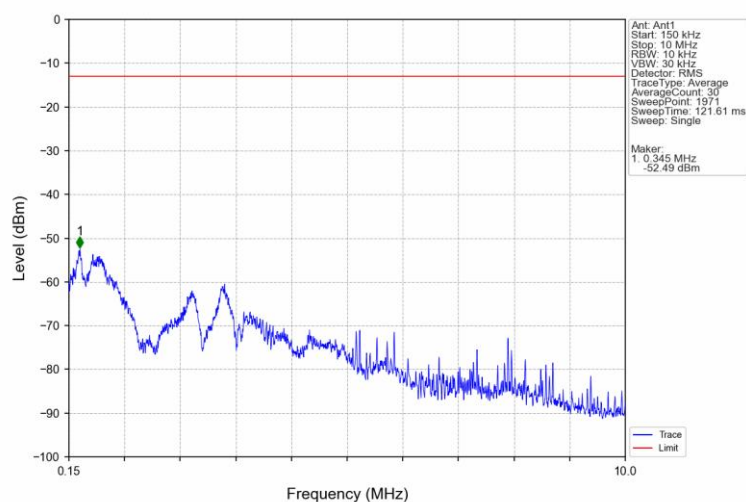
Band4_HSUPA_MCH_1732.6MHz_Subtest 1_NTNV
