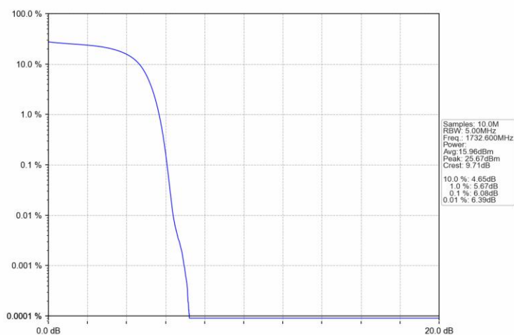
Band4 HSDPA MCH 1732.6MHz Subtest 1 NTNV
