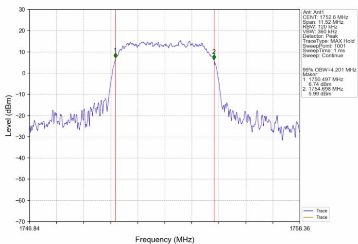
Band4 HSDPA HCH 1752.6MHz Subtest 1 NTNV
