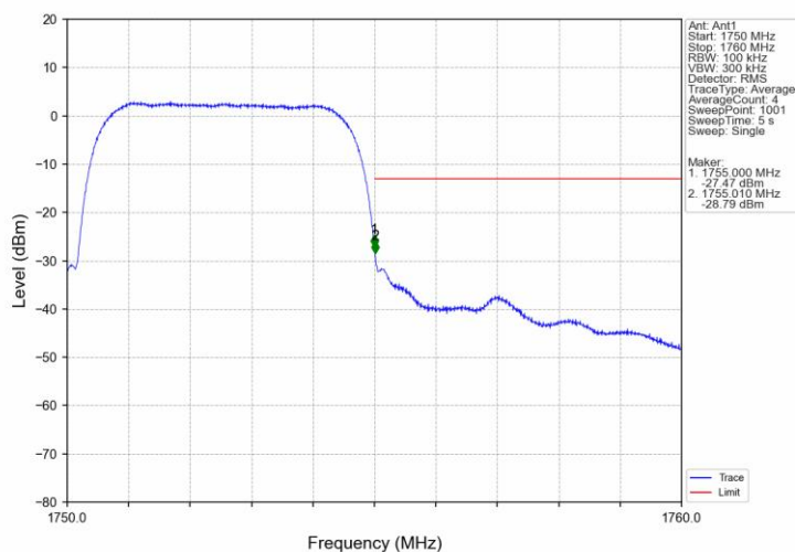
Band4 HSDPA HCH 1752.6MHz Subtest 1 NTNV
