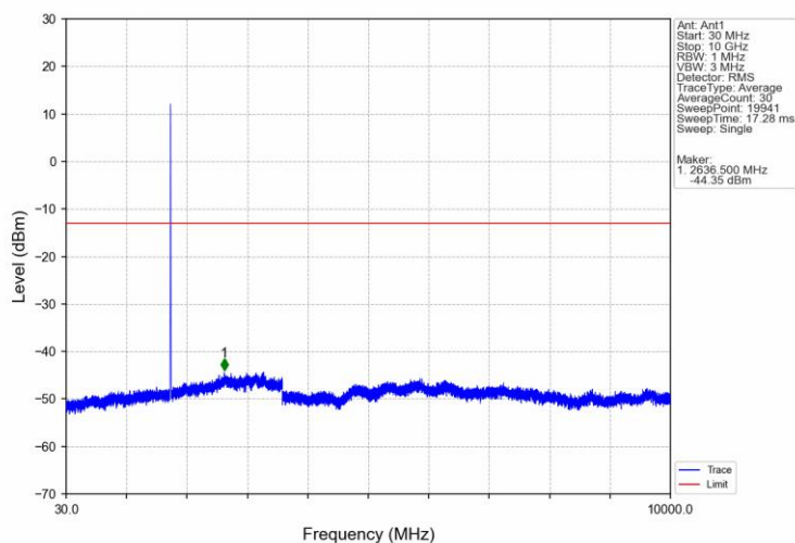
Band4 HSDPA HCH 1752.6MHz Subtest 1 NTNV
