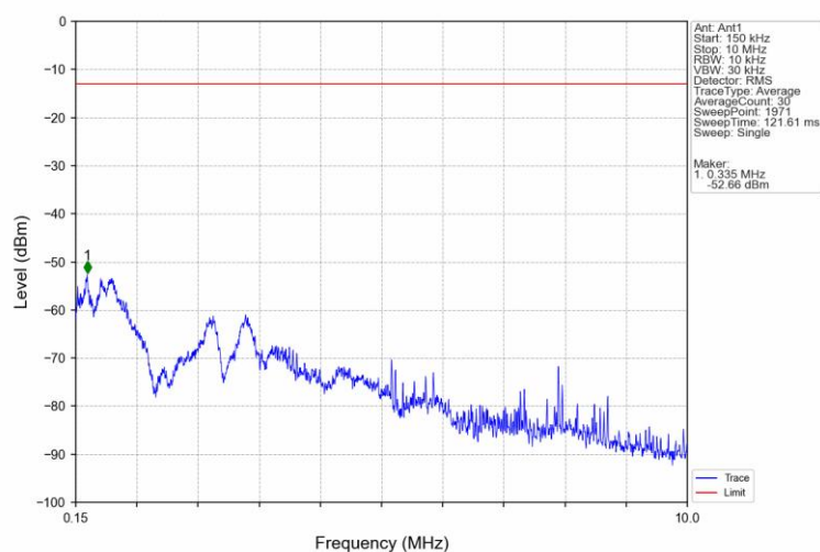
Band4_HSDPA_LCH_1712.4MHz_Subtest 1_NTNV
