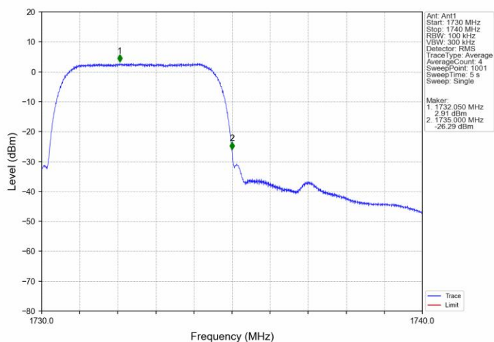
Band4 HSUPA MCH 1732.6MHz Subtest 1 NTNV
