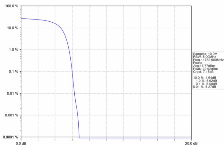
Band4 HSDPA HCH 1752.6MHz Subtest 1 NTNV
