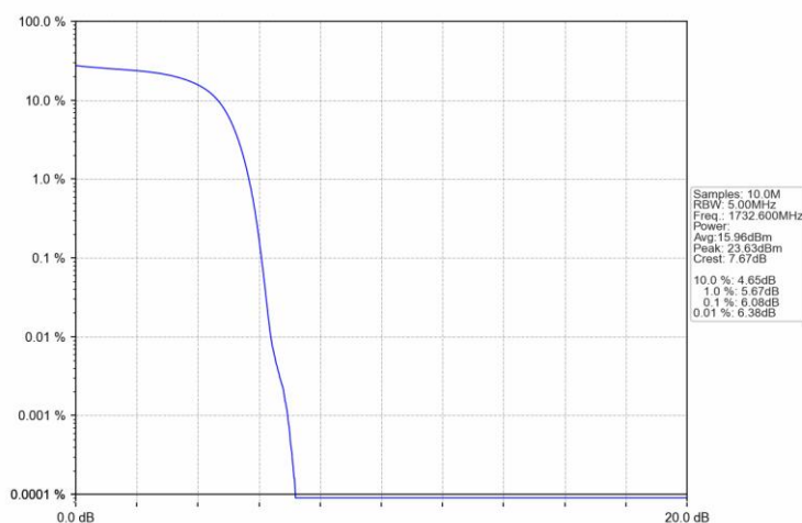
Band4 HSUPA MCH 1732.6MHz Subtest 1 NTVN
