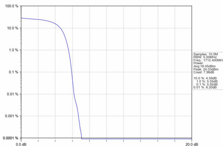
Band4_HSDPA_LCH_1712.4MHz_Subtest 1_NTNV
