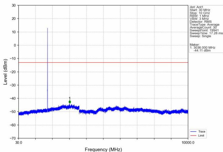
Band4 HSUPA MCH 1732.6MHz Subtest 1 NTNV
