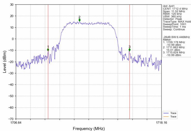
Band4_HSDPA_LCH_1712.4MHz_Subtest 1_NTN
