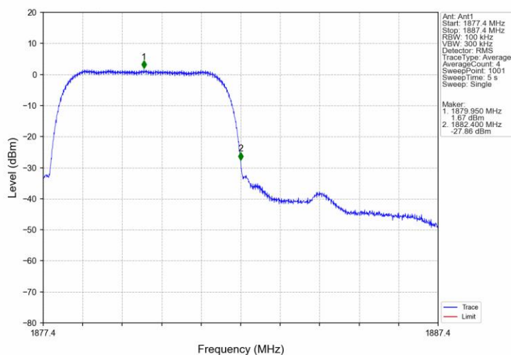
Band2_HSDPA_MCH_1880MHz_Subtest 1_NTNV
