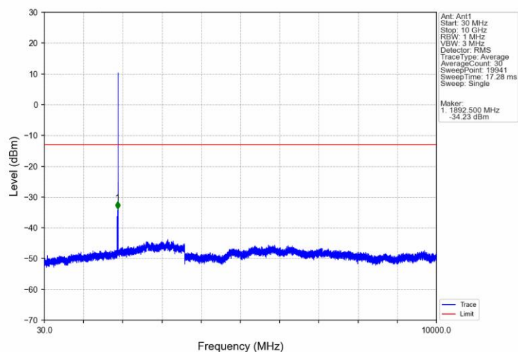
Band2 HSUPA HCH 1907.6MHz Subtest 1 NTV
