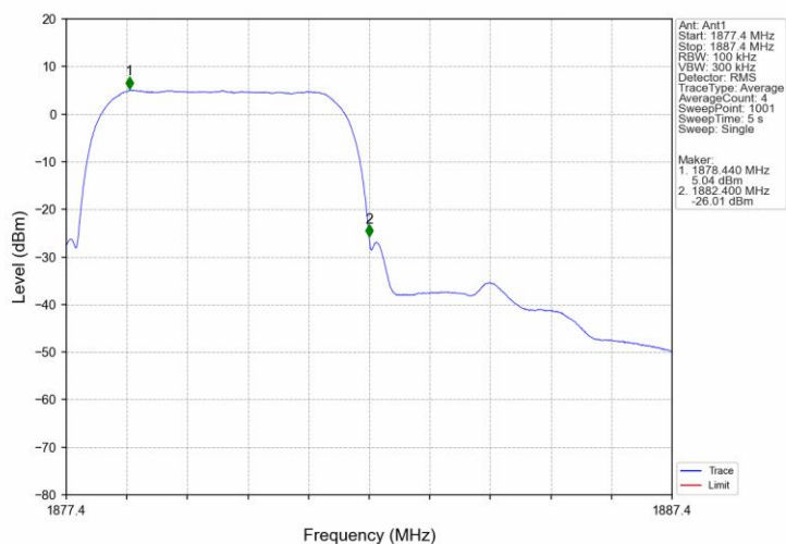
Band2_RMC_MCH_1880MHz_12.2kbps_RMC_NTNV
