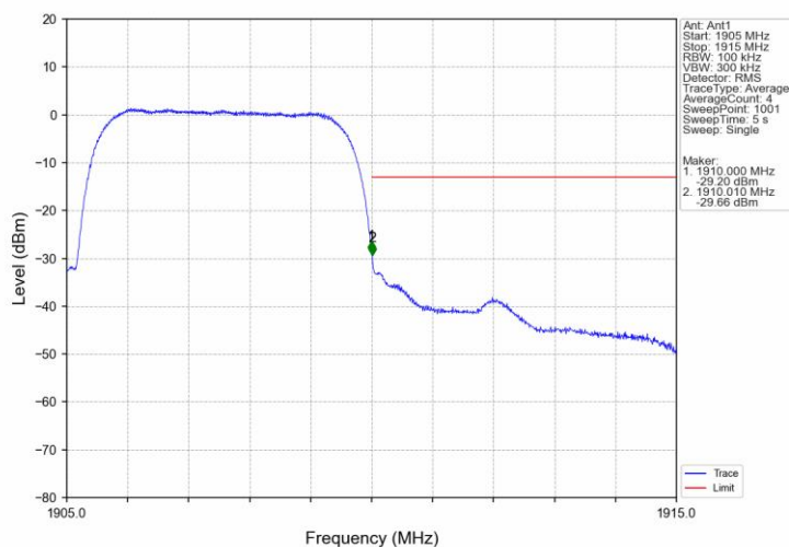
Band2_HSDPA_HCH_1907.6MHz_Subtest 1_NTNV
