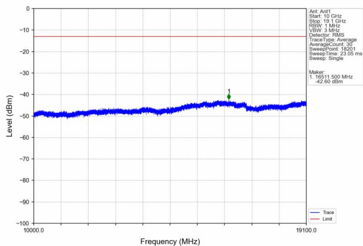
Band2 HSUPA HCH 1907.6MHz Subtest 1 NTV
