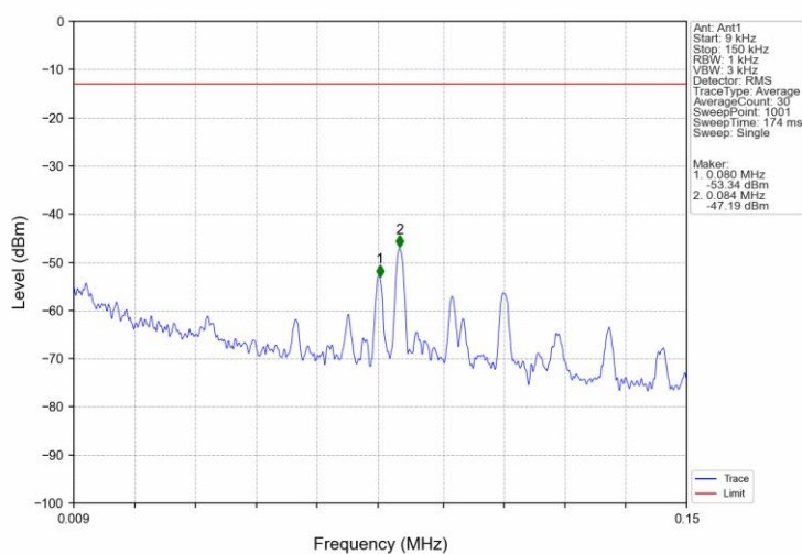
Band2_HSDPA_LCH_1852.4MHz_Subtest 1_NTNV
