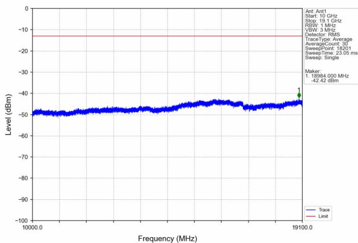
Band2 HSDPA HCH 1907.6MHz Subtest 1 NTNV
