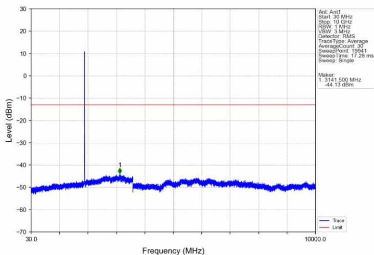
Band2 HSDPA HCH 1907.6MHz Subtest 1 NTNV
