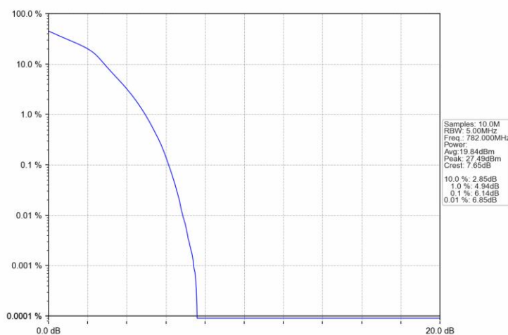
Band13 5MHz 16QAM MCH 782MHz RB 25 0 NTNV
