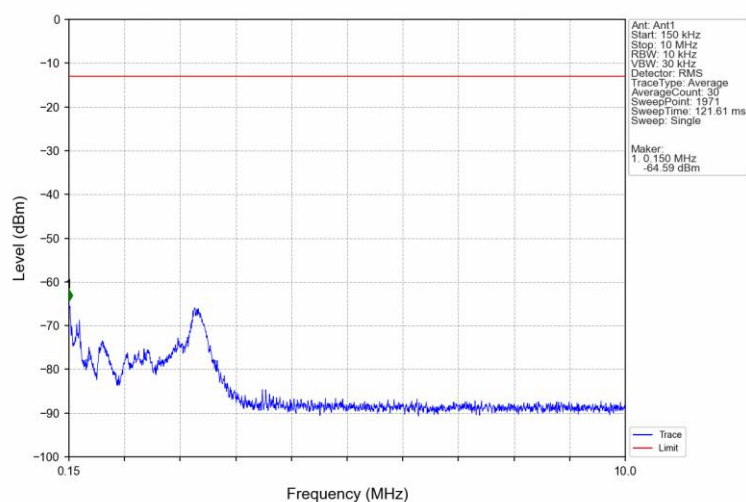
Band12_5MHz_16QAM_LCH_701.5MHz_RB_1_0_NTNV
