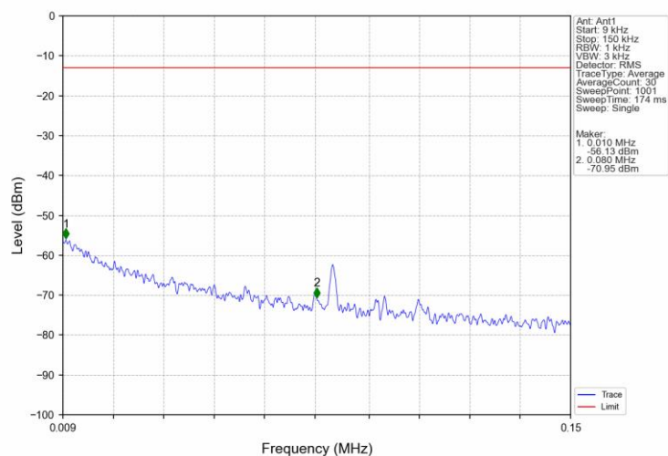
Band12 10MHz QPSK HCH 711MHz RB 1 0 NTN
