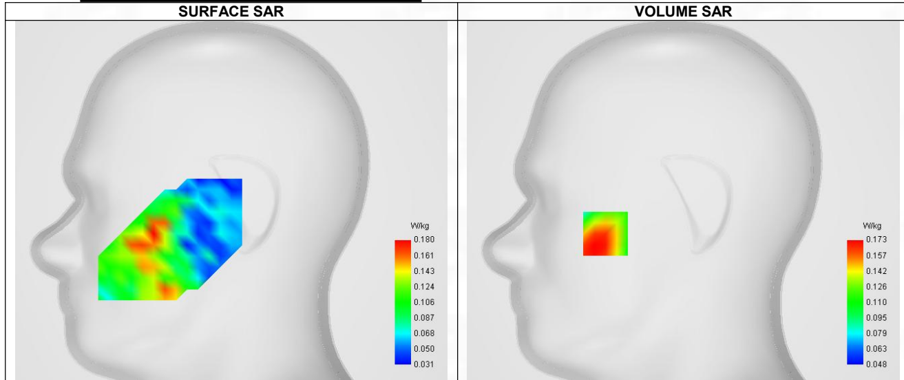
Maximum location: X=-56.00, Y=-24.00 ; SAR Peak: 0.23 W/kg
