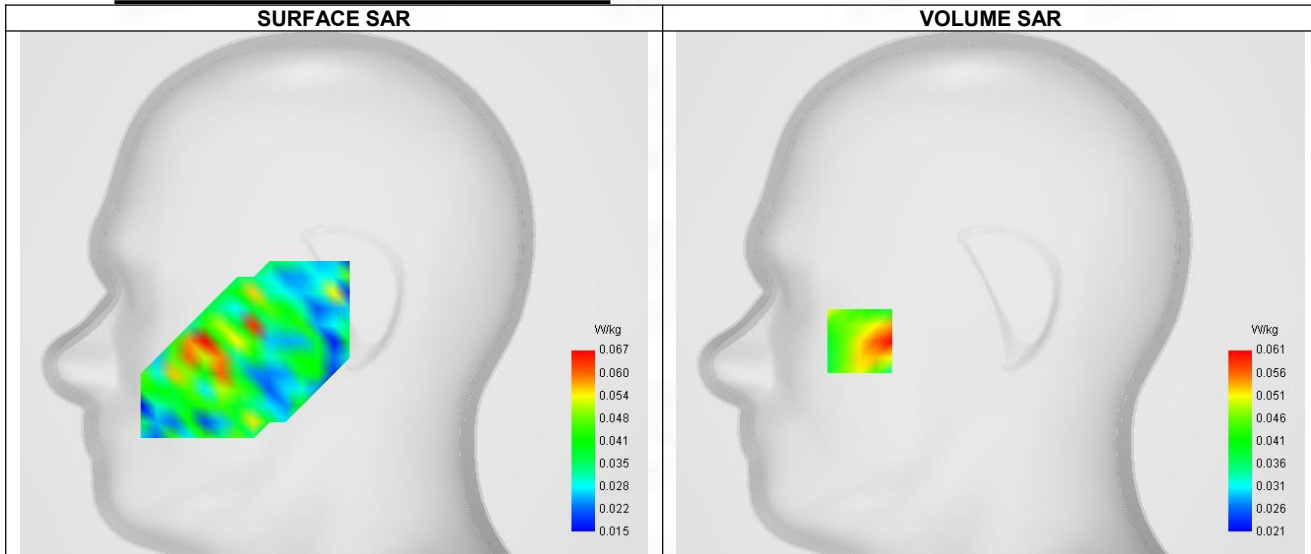
Maximum location: X=-65.00, Y=-24.00 ; SAR Peak: 0.08 W/kg
