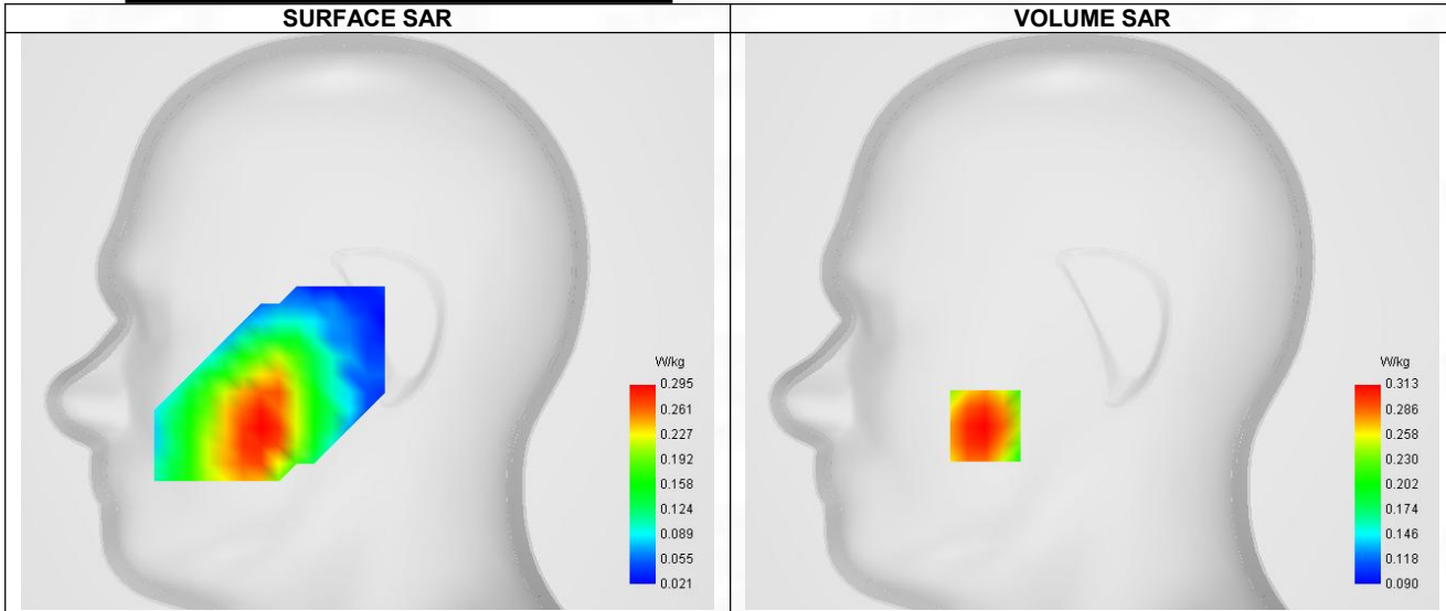
Maximum location: X=-48.00, Y=-47.00 ; SAR Peak: 0.36 W/kg
