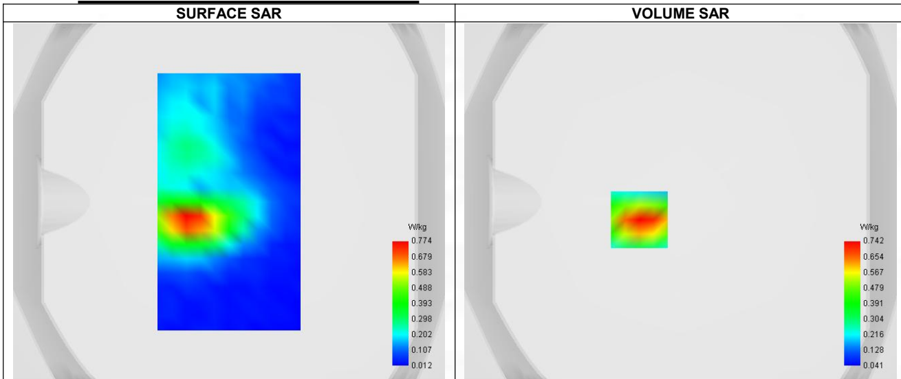
Maximum location: X=-23.00, Y=-10.00 ; SAR Peak: 1.07 W/kg
