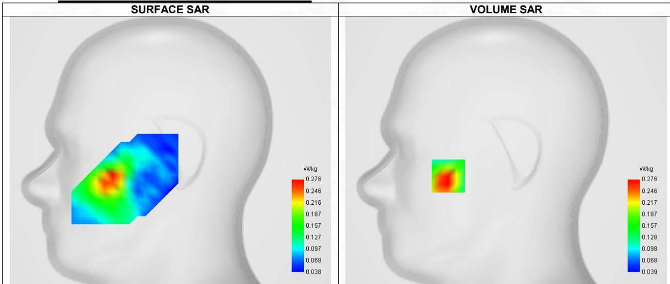
Maximum location: X=-56.00, Y=-25.00 ; SAR Peak: 0.40 W/kg
