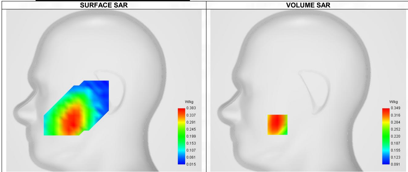
Maximum location: X=-49.00, Y=-55.00 ; SAR Peak: 0.39 W/kg
