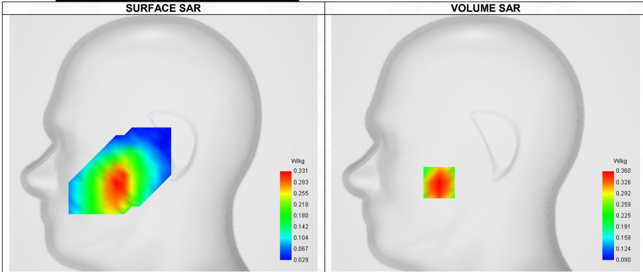
Maximum location: X=-47.00, Y=-40.00 ; SAR Peak: 0.43 W/kg
