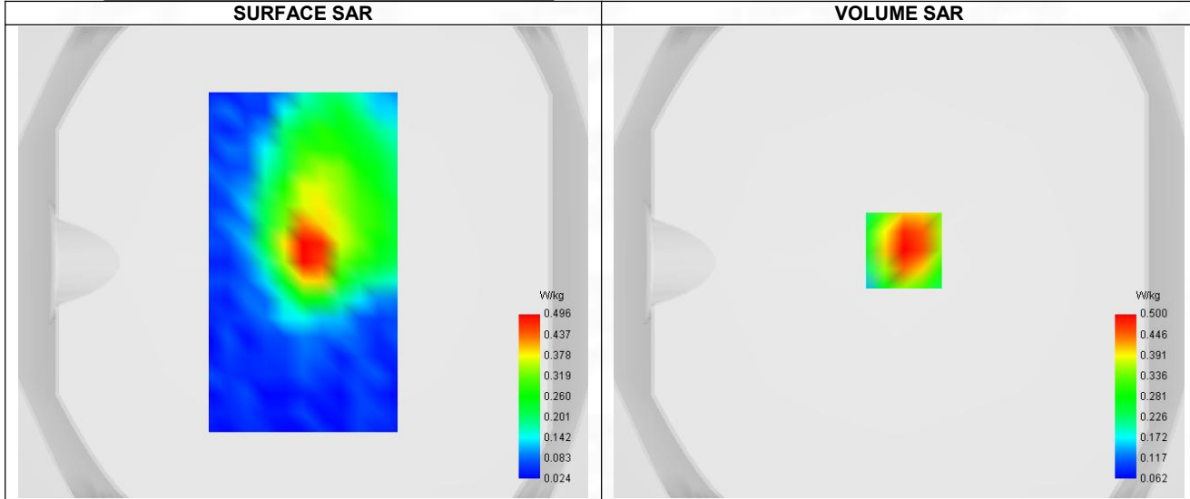
Maximum location: X=2.00, Y=5.00 ; SAR Peak: 0.72 W/kg
