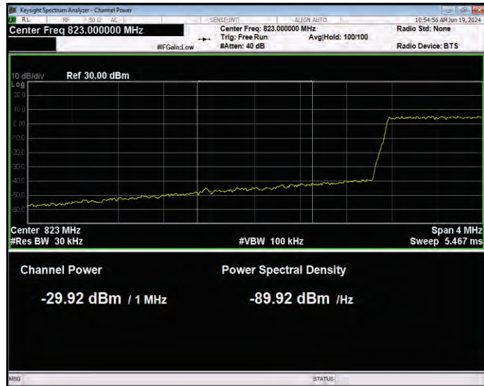
Band26(824-849) 16QAM BW=1.4MHz Channel=26797 RB Size=6 Position=#0 Normal
