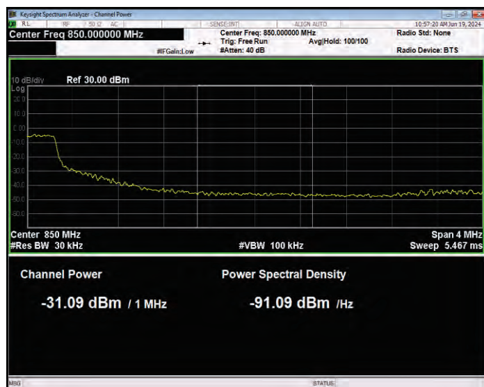
Band26(824-849) QPSK BW=15MHz Channel=26965 RB Size=75 Position=#0 Normal
