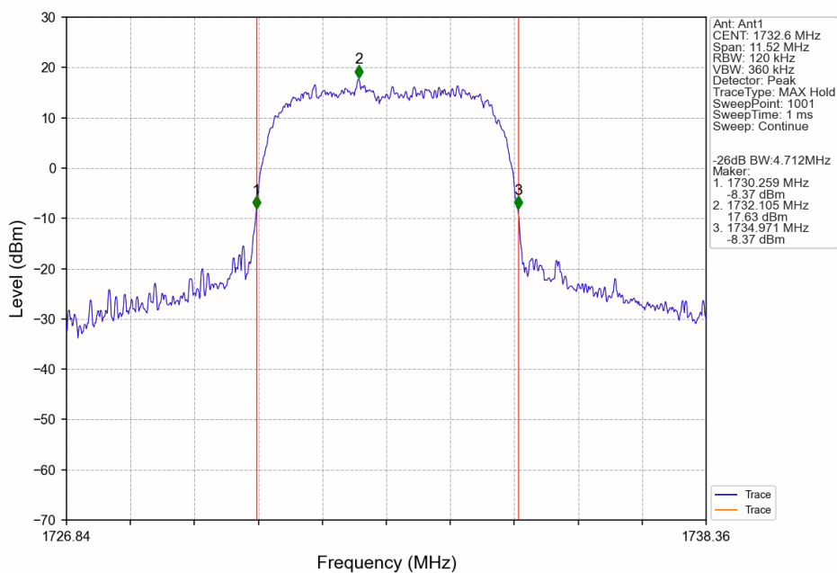
Band4 HSUPA MCH 1732.6MHz Subtest 1 NTN
