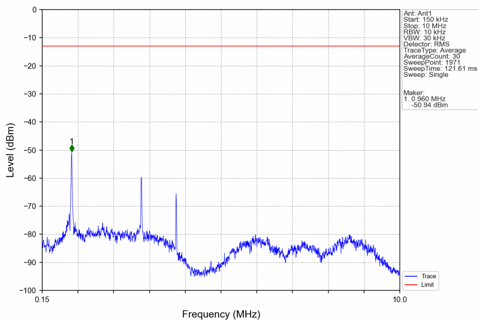
Band4 HSDPA LCH 1712.4MHz Subtest 1 NTV
