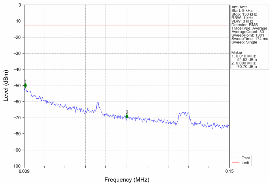
Band4 HSDPA LCH 1712.4MHz Subtest 1 NTV
