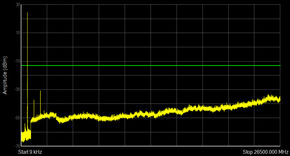
Band71 QPSK BW=5MHz Channel=133147 RB Size=1 Position=#0
