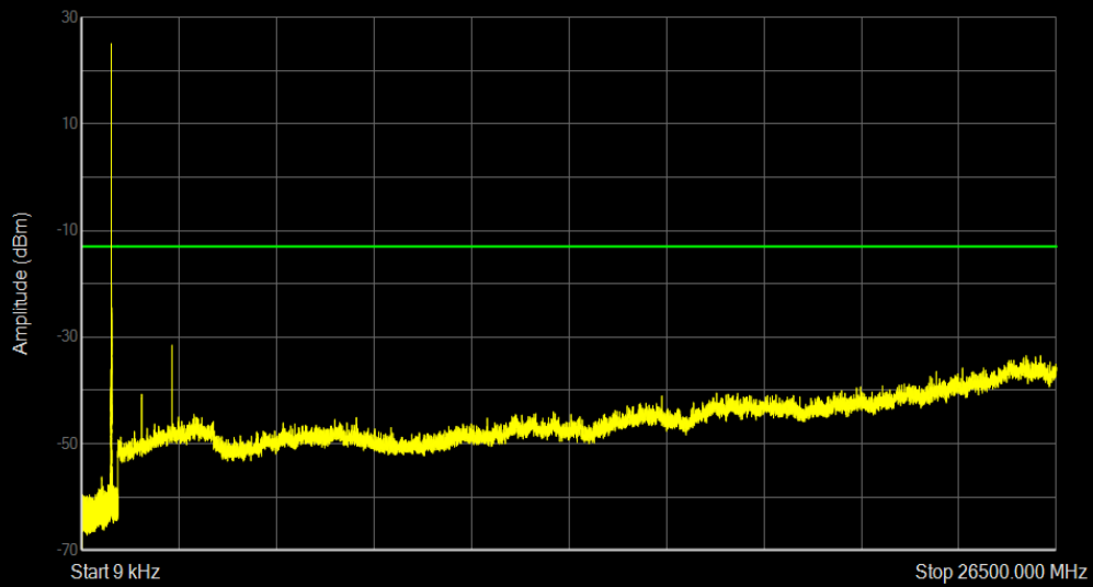
Band5 QAM16 BW=5MHz Channel=20425 RB Size=1 Position=#0
