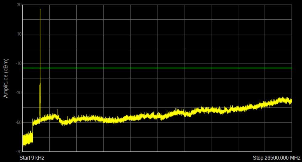
Band66 QAM16 BW=15MHz Channel=132322 RB Size=1 Position=#0
