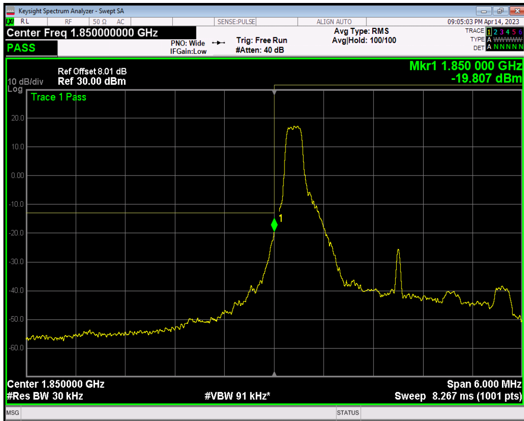
Band25 QPSK BW=3MHz Channel=26055 RB Size=1 Position=#Max
