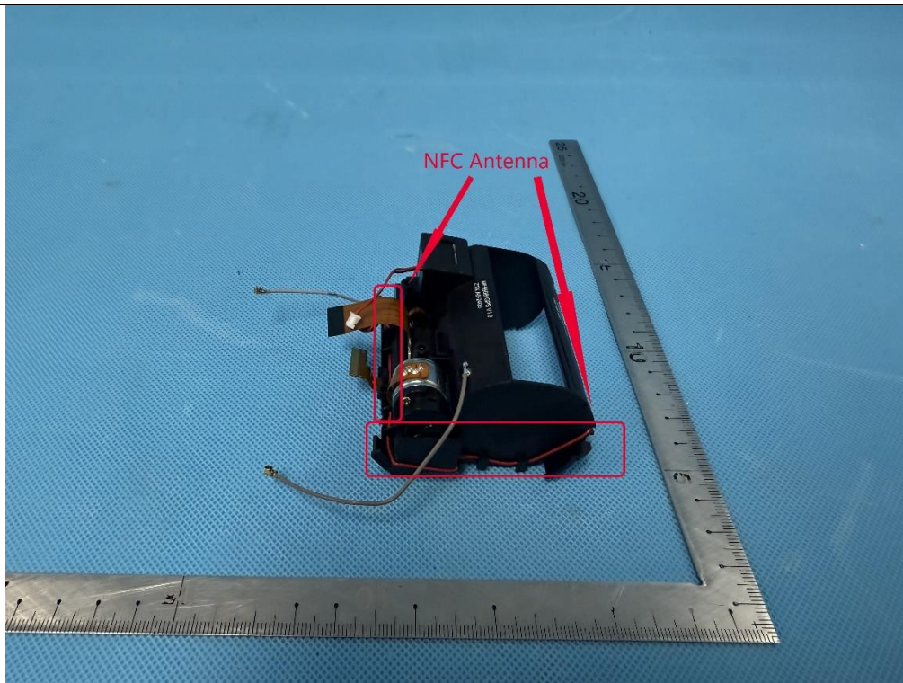
EUT Photo(12) Antenna close-up
