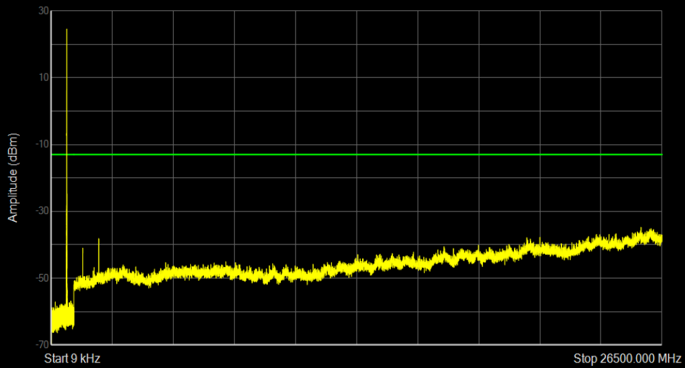
Band71 16QAM BW=5MHz Channel=133447 RB Size=1 Position=#0
