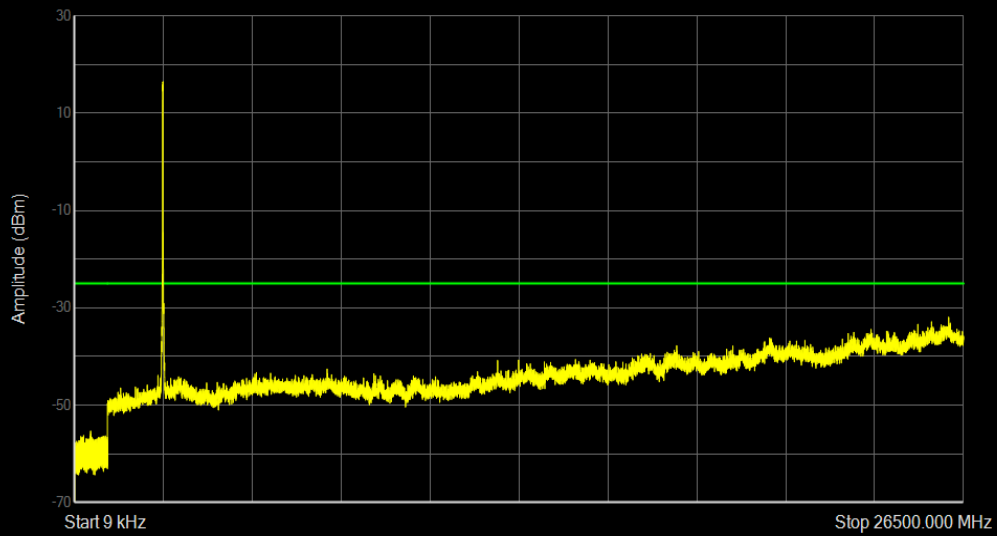
Band41 16QAM BW=15MHz Channel=41165 RB Size=75 Position=#0
