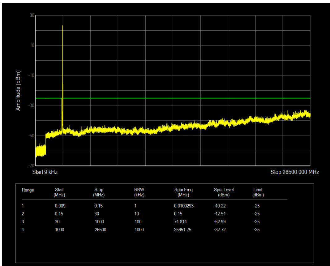
Band41 16QAM BW=20MHz Channel=41140 RB Size=1 Position=#0
