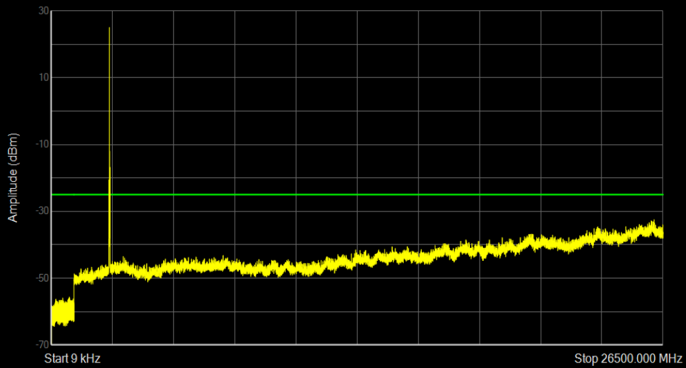
Band41 16QAM BW=15MHz Channel=40115 RB Size=1 Position=#0
