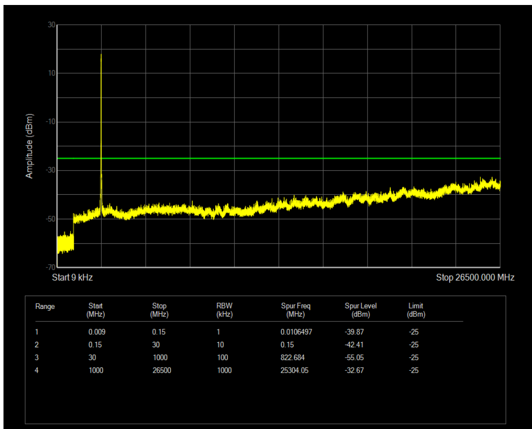
Band41 16QAM BW=15MHz Channel=41165 RB Size=1 Position=#0
