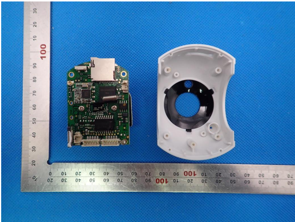
OPEN VIEW OF EUT(FIGURE 6)
