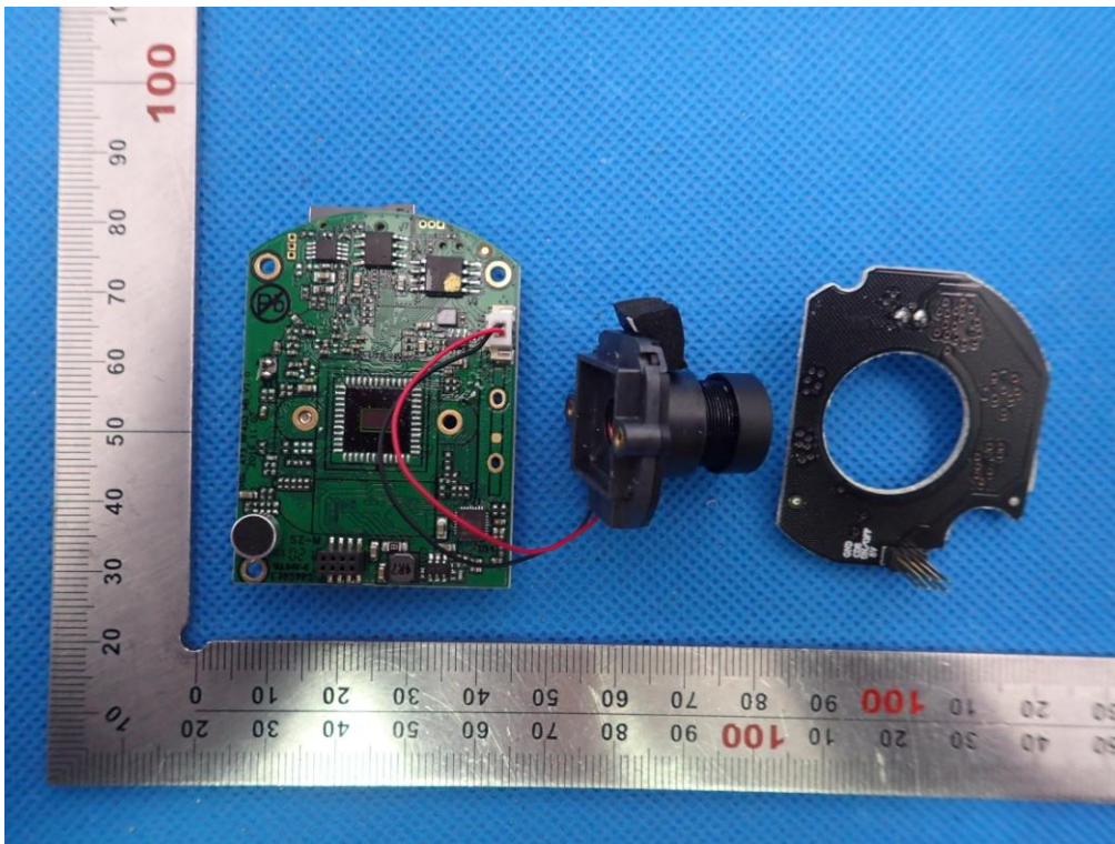
OPEN VIEW OF EUT(FIGURE 7)
