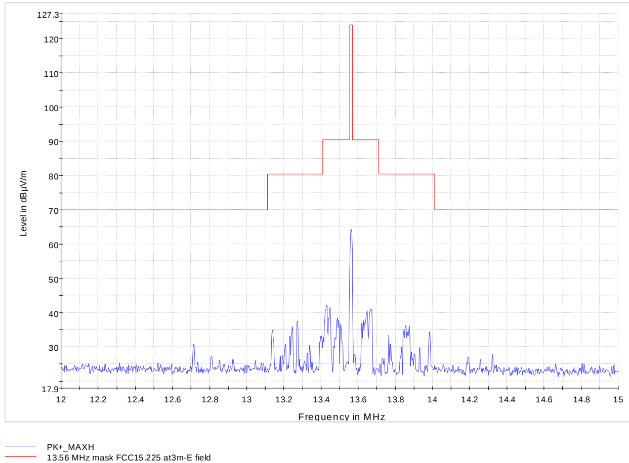
Figure 8.3-2: Field strength within 13.56 MHz mask
