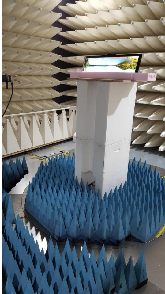
Figure B8. Radiated Emission test setup3 HR (18-26GHz)
