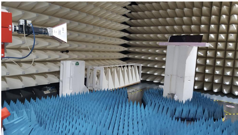
Figure B7. Radiated Emission test setup2 HR (1-18GHz)
