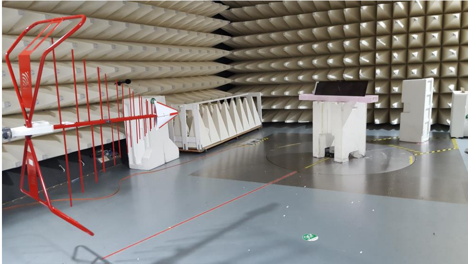
Figure B6. Radiated Emission test setup1 LR (0.03-1GHz)
