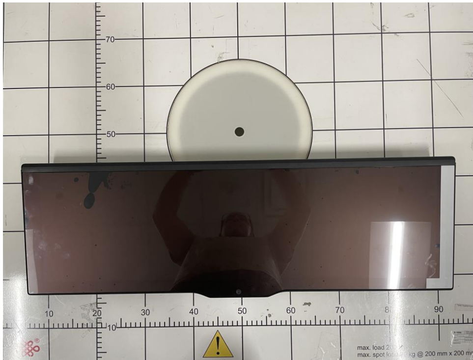
Figure B3. Front View of Conducted Sample
