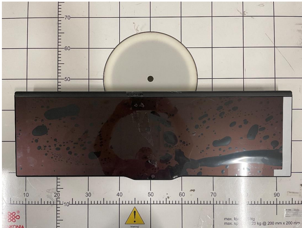
Figure B1. Front View of Radiated Sample
