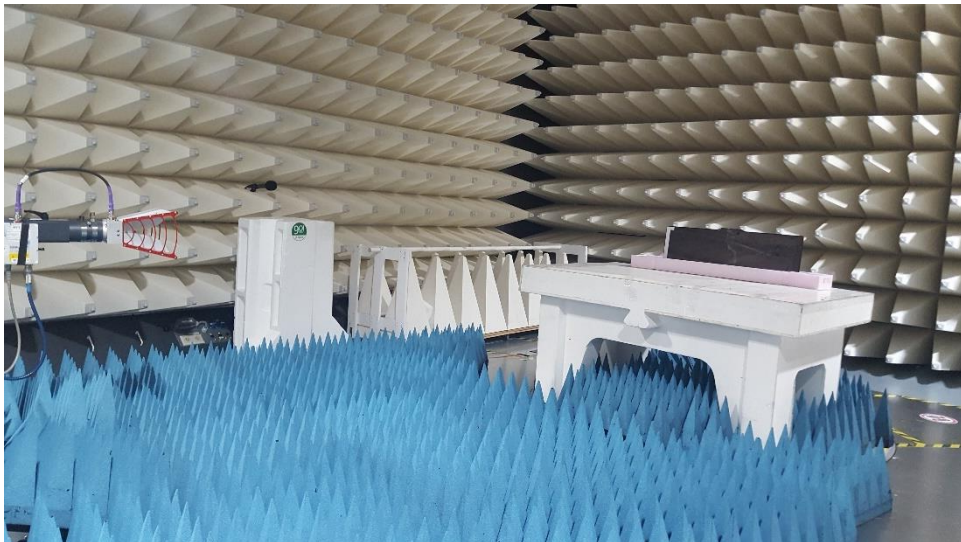
Figure B5. High Range Radiated Emission test setup 1-18GHz
