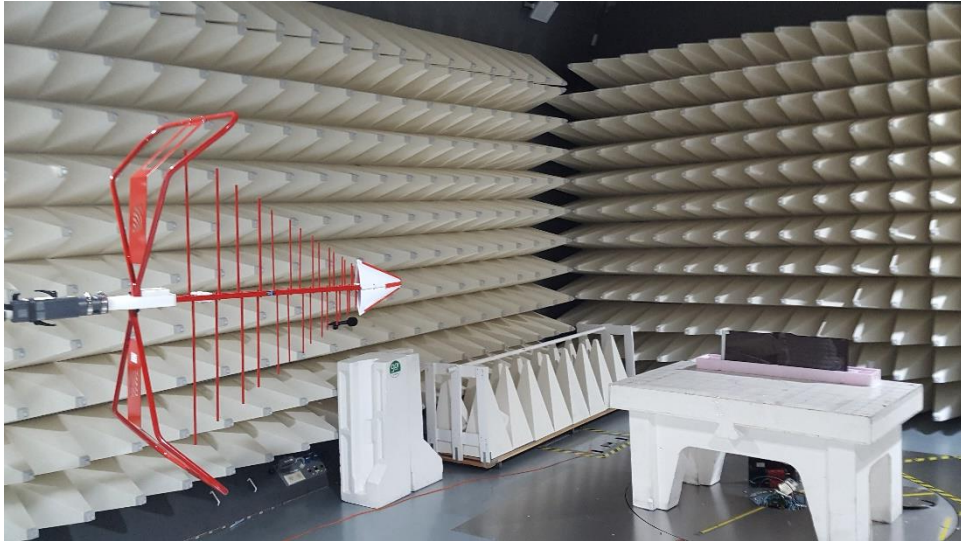
Figure B4. Low Range Radiated Emission test setup
