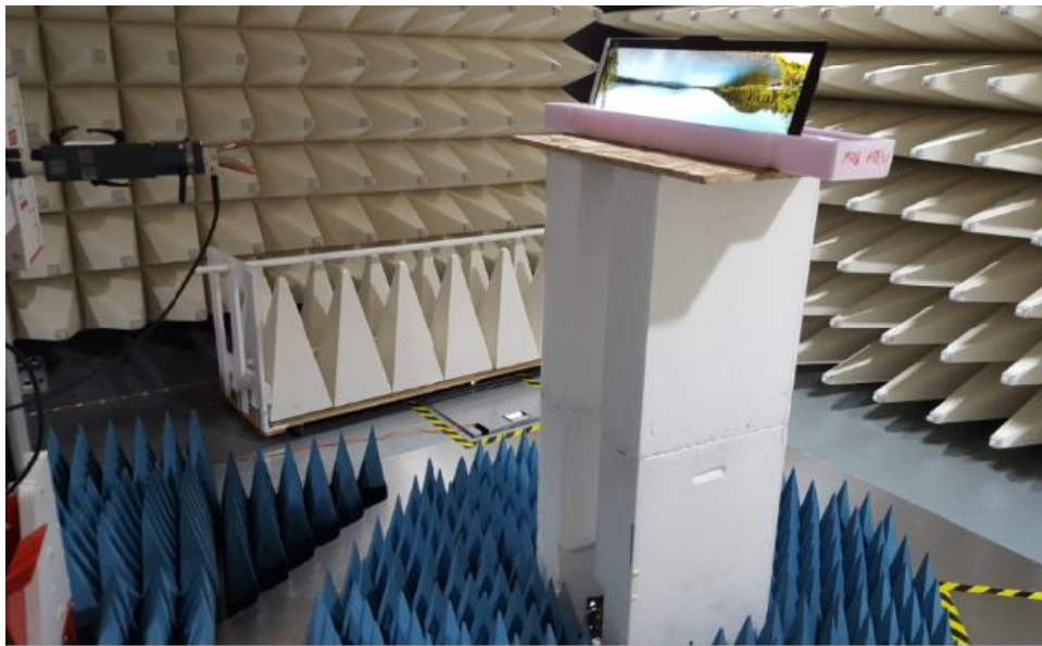
Figure B6. Radiated emission Setup 3
