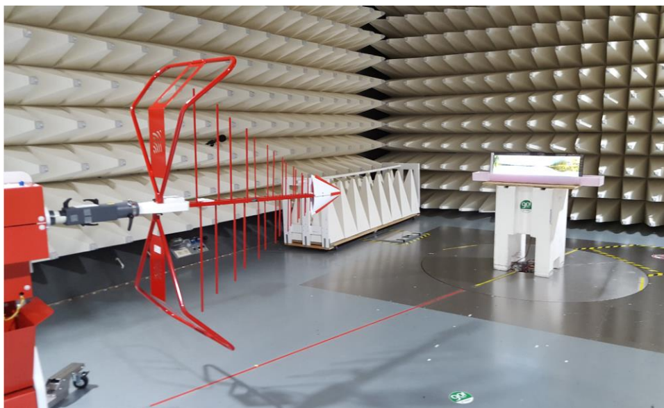
Figure B4. Radiated emission Setup 1
