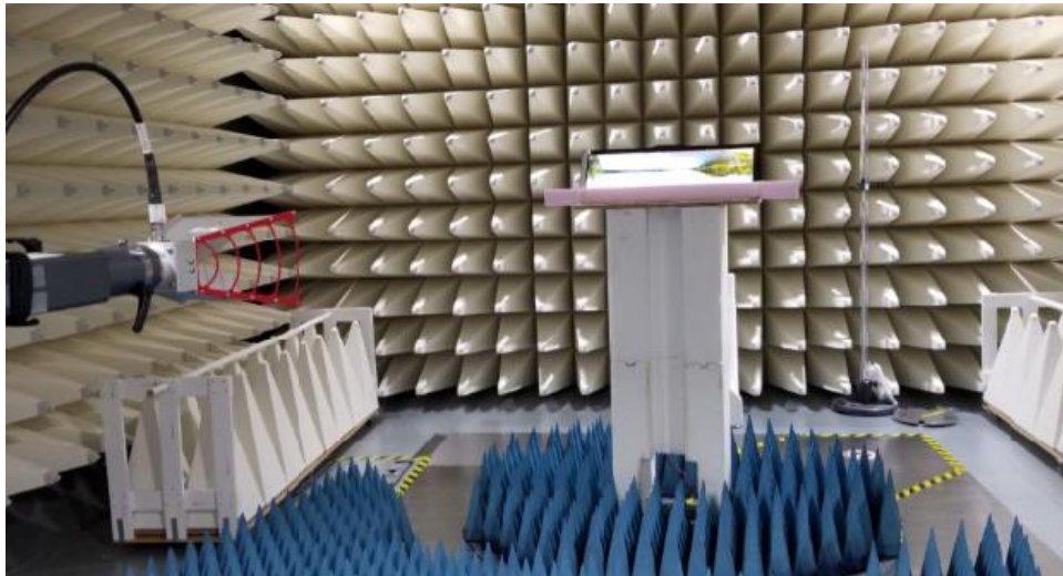
Figure B5. Radiated emission Setup 2
