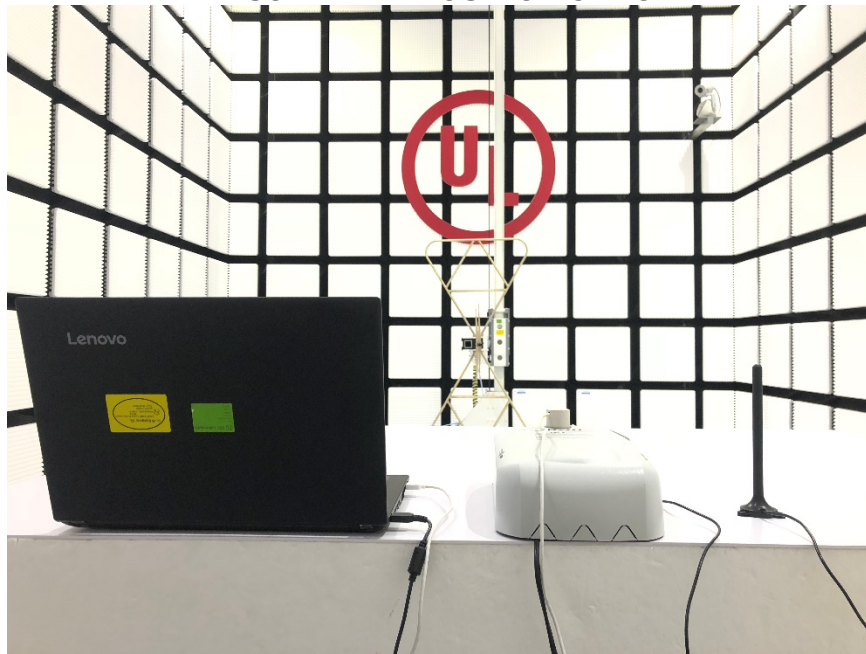
MEASUREMENT POSITION OF LORA
