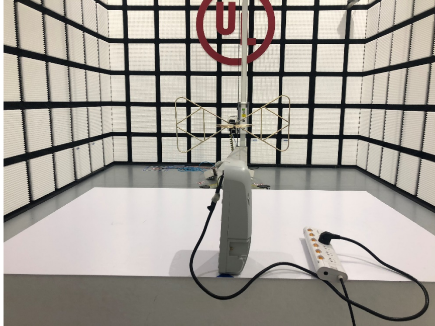
MEASUREMENT POSITION OF WCDMA Band5
