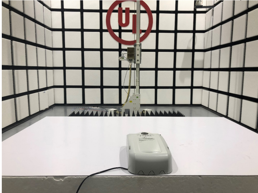
MEASUREMENT POSITION OF WCDMA Band 5 (Z axis)
