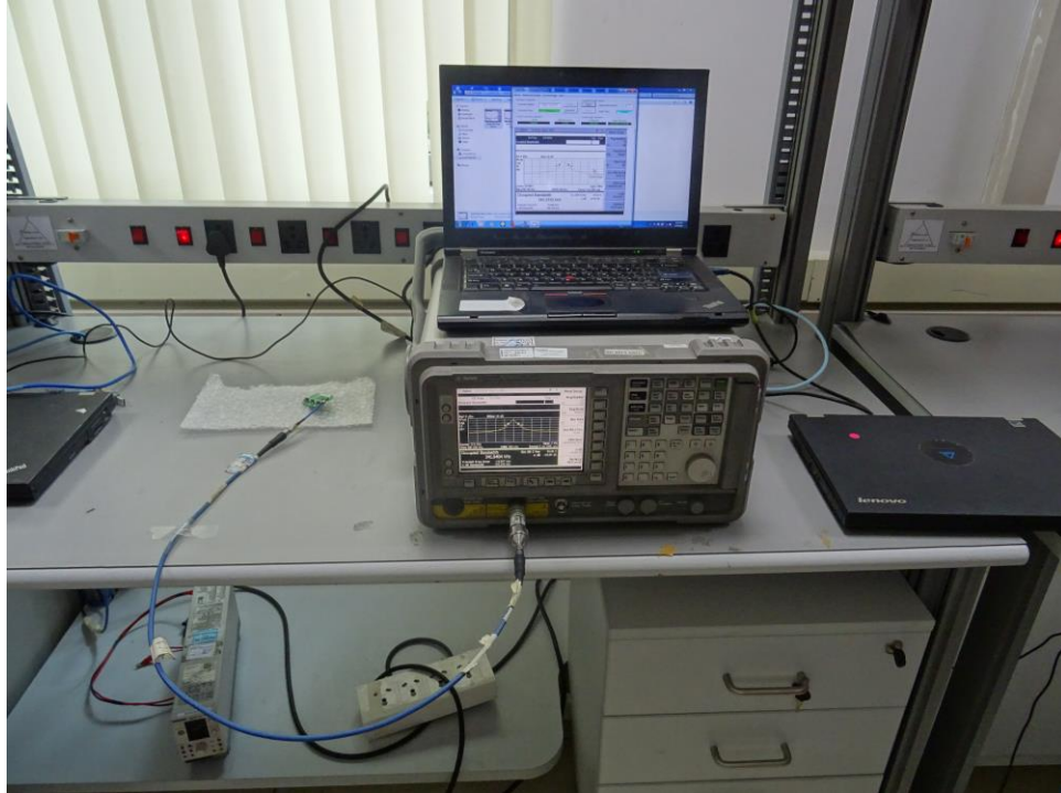
Test Setup: Antenna Port Conducted Measurement
