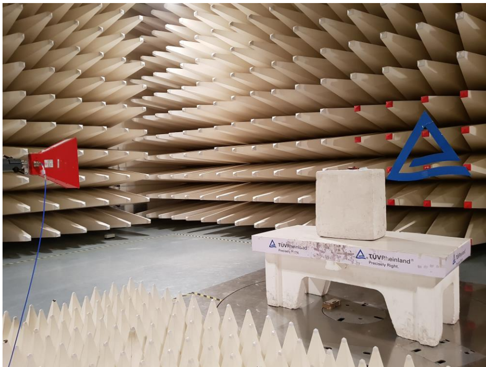
Test Setup: Antenna Horizontal Polarization
