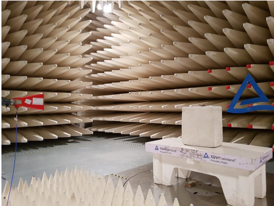
Test Setup: Antenna Vertical Polarization
