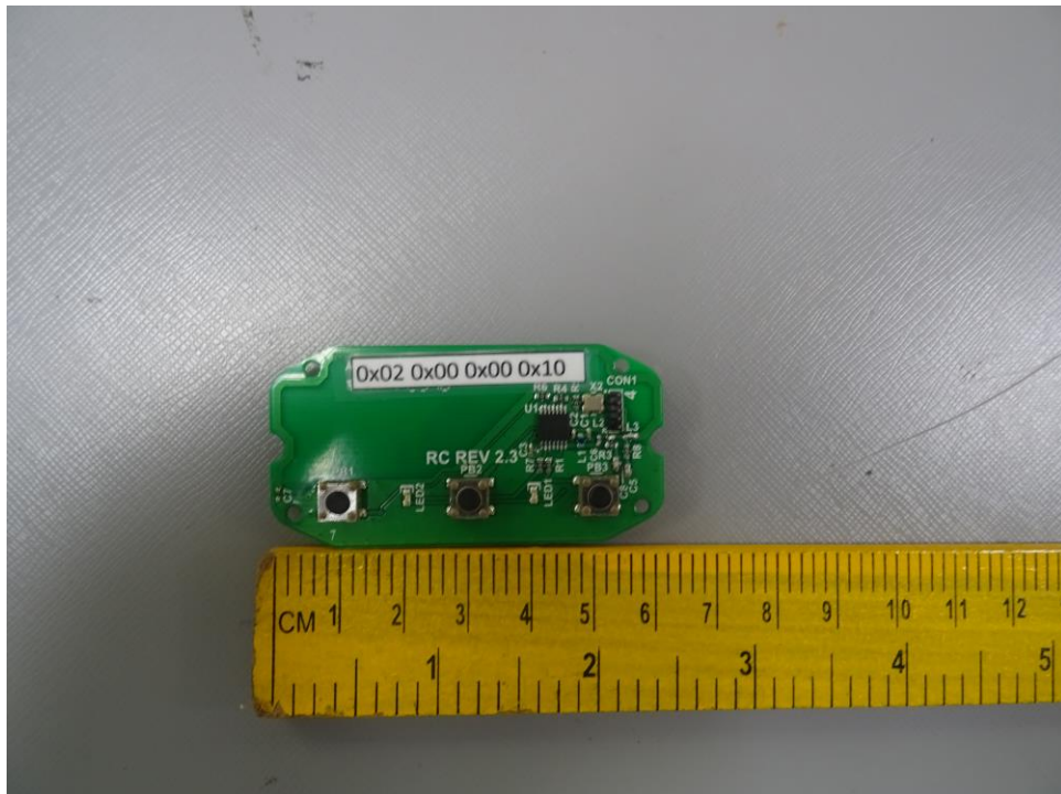
PCB Dimensional Front View
