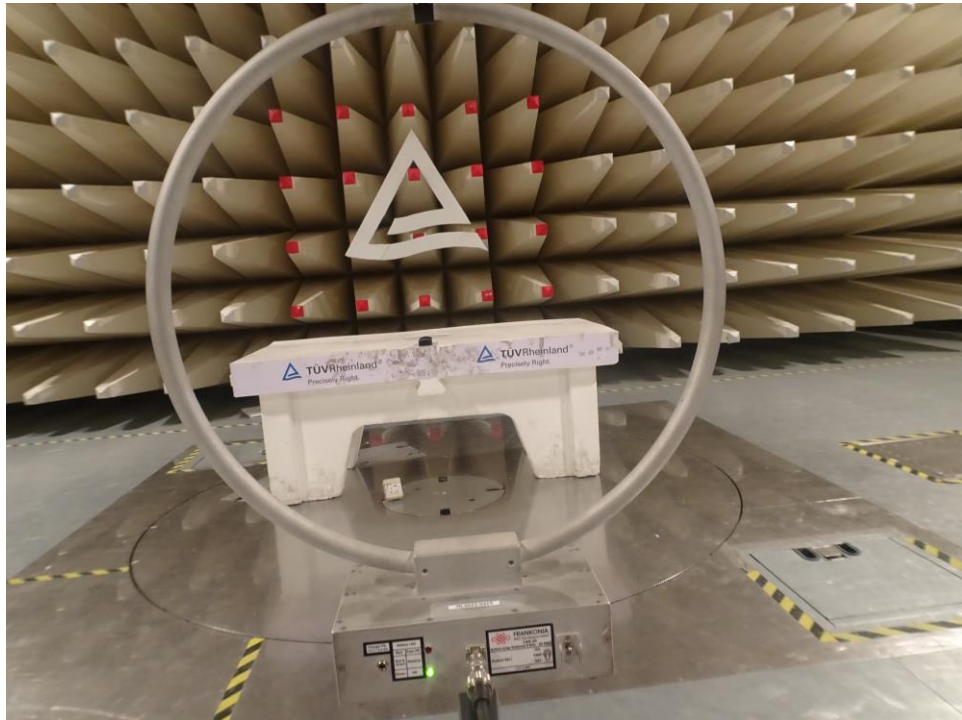
Test Setup: 9 kHz-30 MHz, Antenna Parallel Polarization
