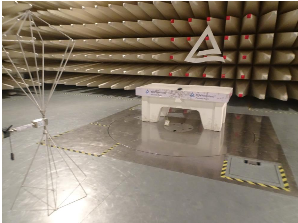
Test Setup: 30MHz-200MHz, Antenna Vertical Polarization
