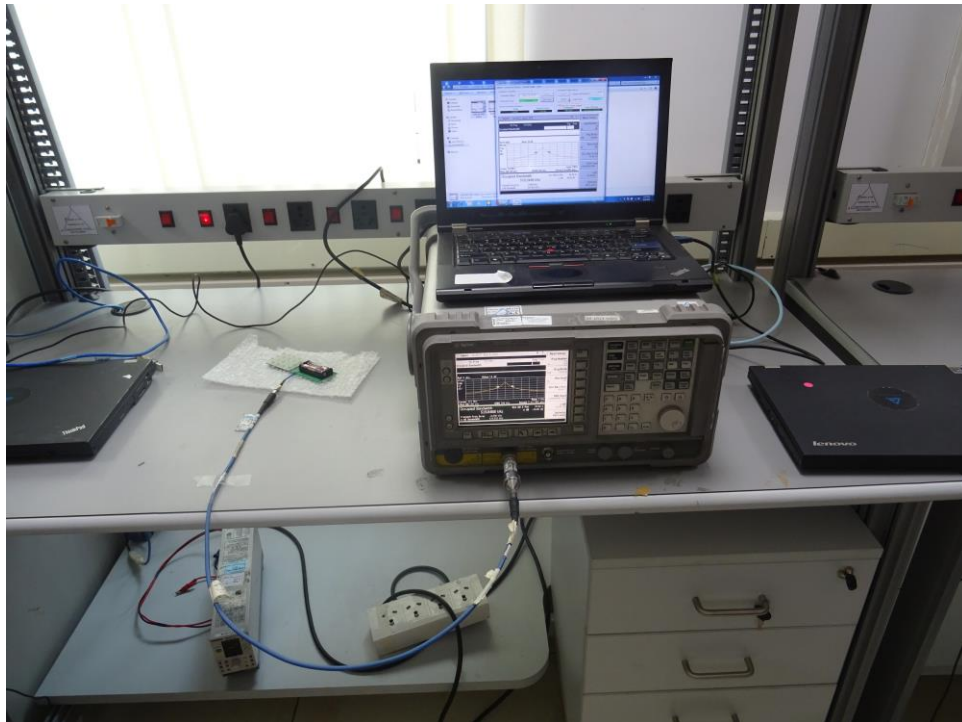
Test Setup: Antenna Port Conducted Mesrurement
