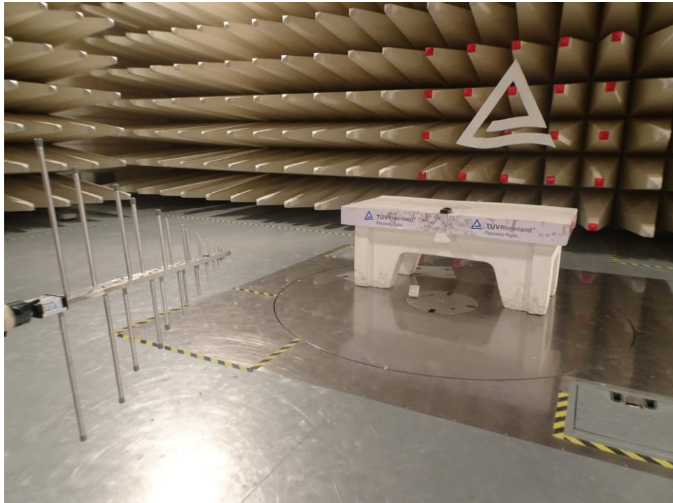
Test Setup: 200MHz-1GHz, Antenna Vertical Polarization
