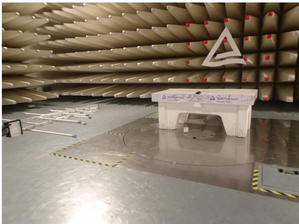
Test Setup: 200MHz-1GHz, Antenna Horizontal Polarization
