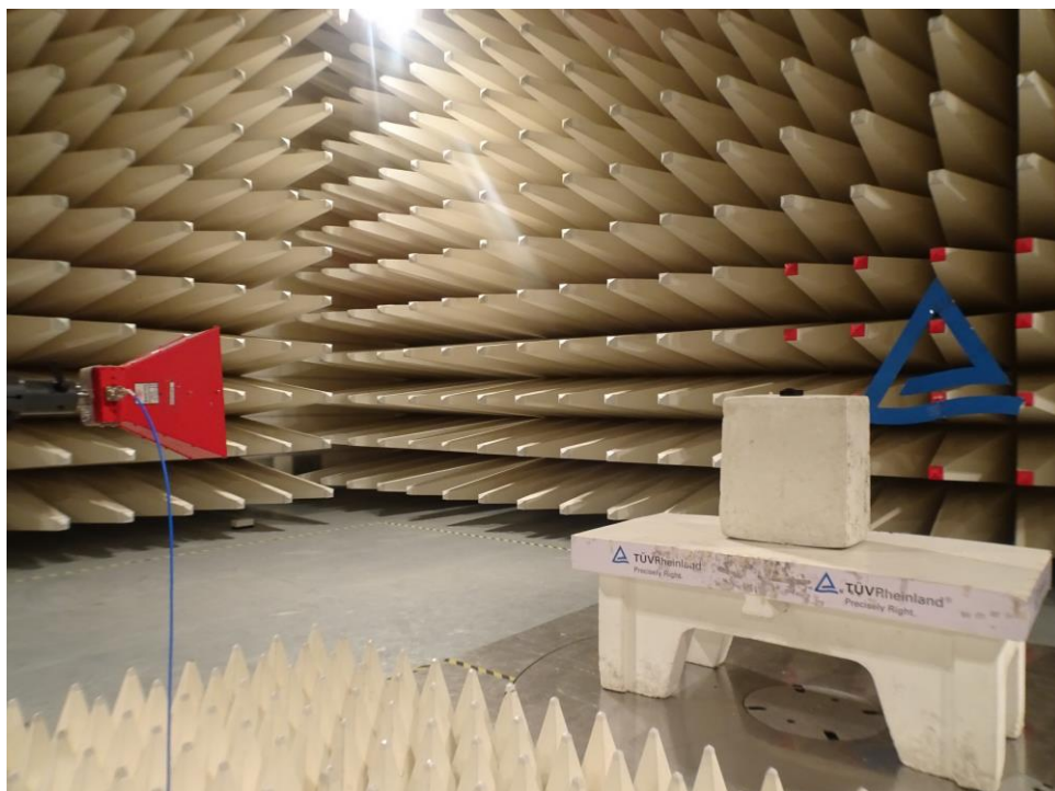
Test Setup: Above 1GHz, Antenna Horizontal Polarization
