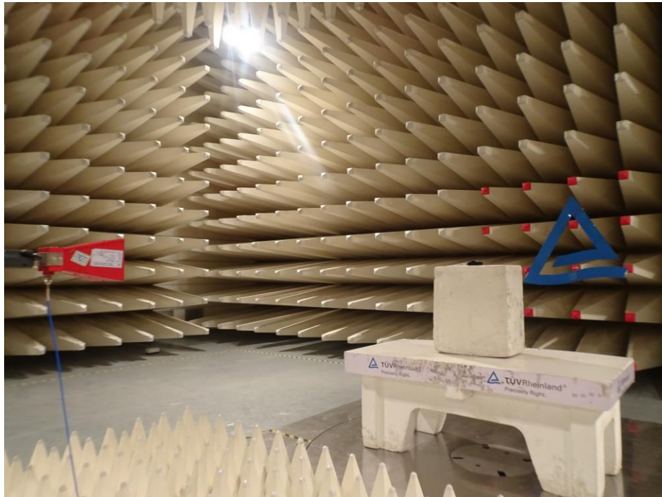
Test Setup: Above 1GHz, Antenna Vertical Polarization
