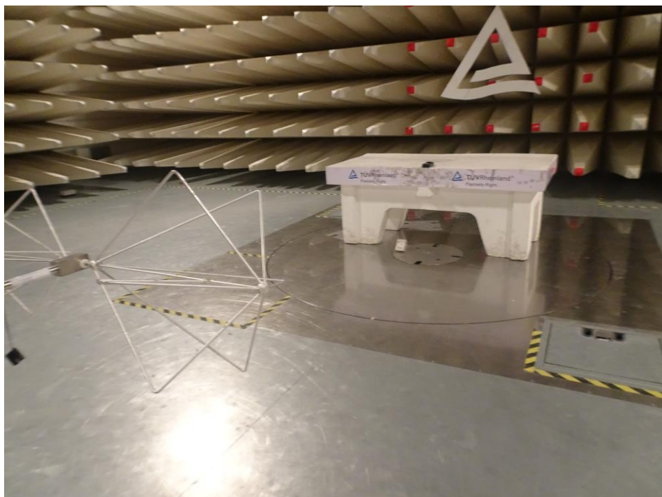
Test Setup: 30MHz-200MHz, Antenna Horizontal Polarization
