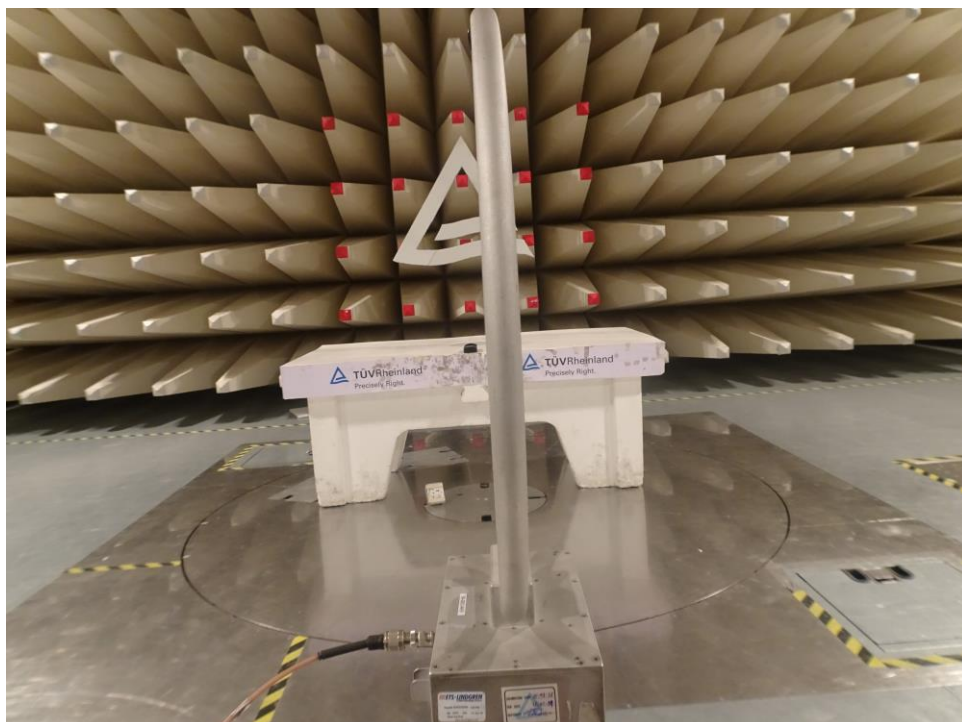
Test Setup: 9 kHz-30 MHz, Antenna Perpendicular Polarization
