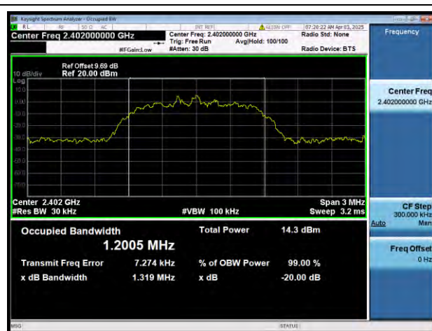
Bluetooth For Classic 2-DH5 2402MHz
