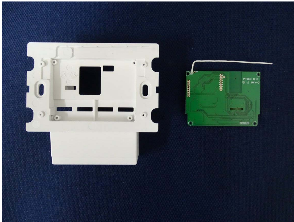
(25) EUT Photo
