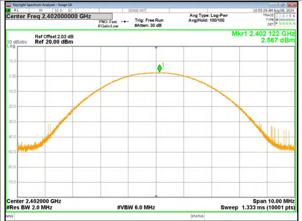
Peak Power NVNT 2-DH5 2402MHz Ant2
