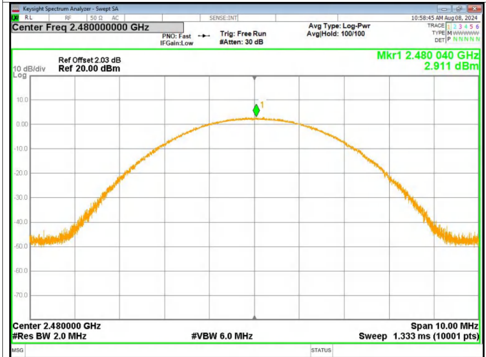
Peak Power NVNT 2-DH5 2480MHz Ant2
