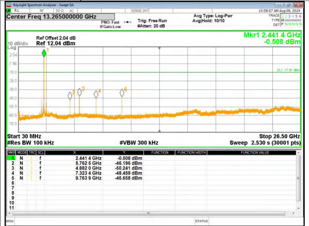
Tx. Spurious NVNT 2-DH5 2441MHz Ant2 Emission
