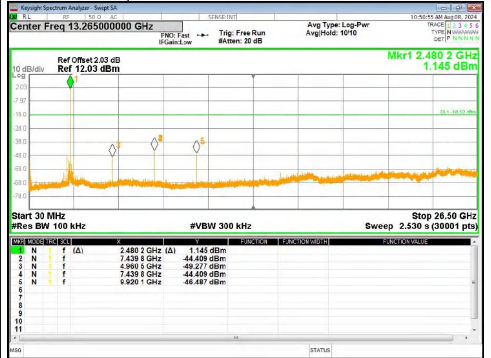
Tx. Spurious NVNT 1-DH5 2480MHz Ant2 Emission
