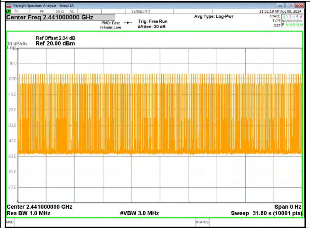
Dwell NVNT 3-DH1 2441MHz Ant2 Accumulated
