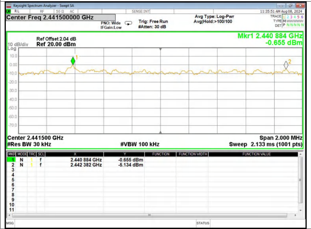
CFS NVNT 2-DH5 2441MHz Ant2
