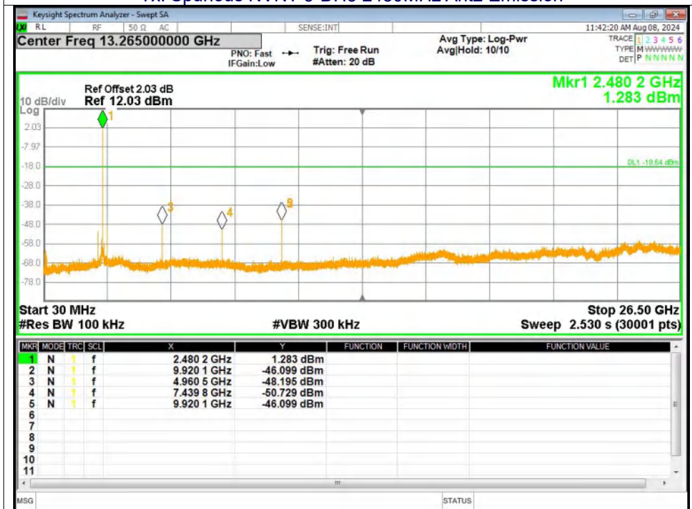
Tx. Spurious NVNT 3-DH5 2480MHz Ant2 Emission
