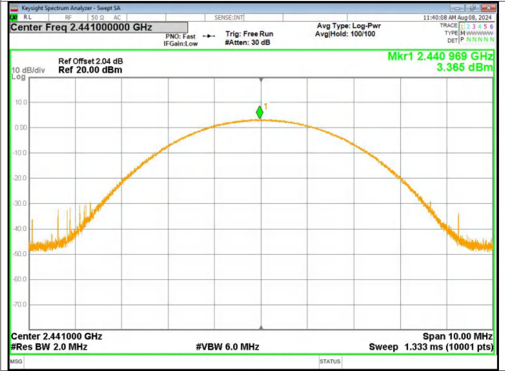
Peak Power NVNT 3-DH5 2441MHz Ant2
