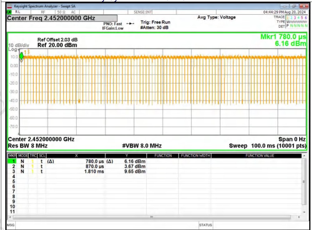
Duty Cycle NVNT n40 2452MHz Ant2
