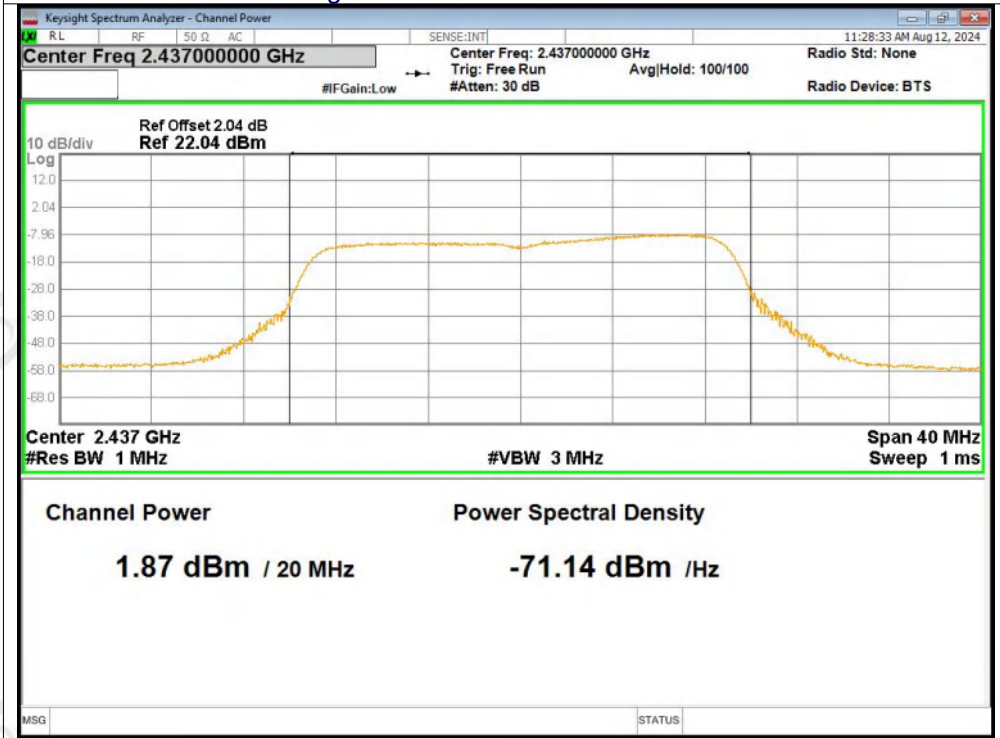
Average Power NVNT n20 2437MHz Ant2
