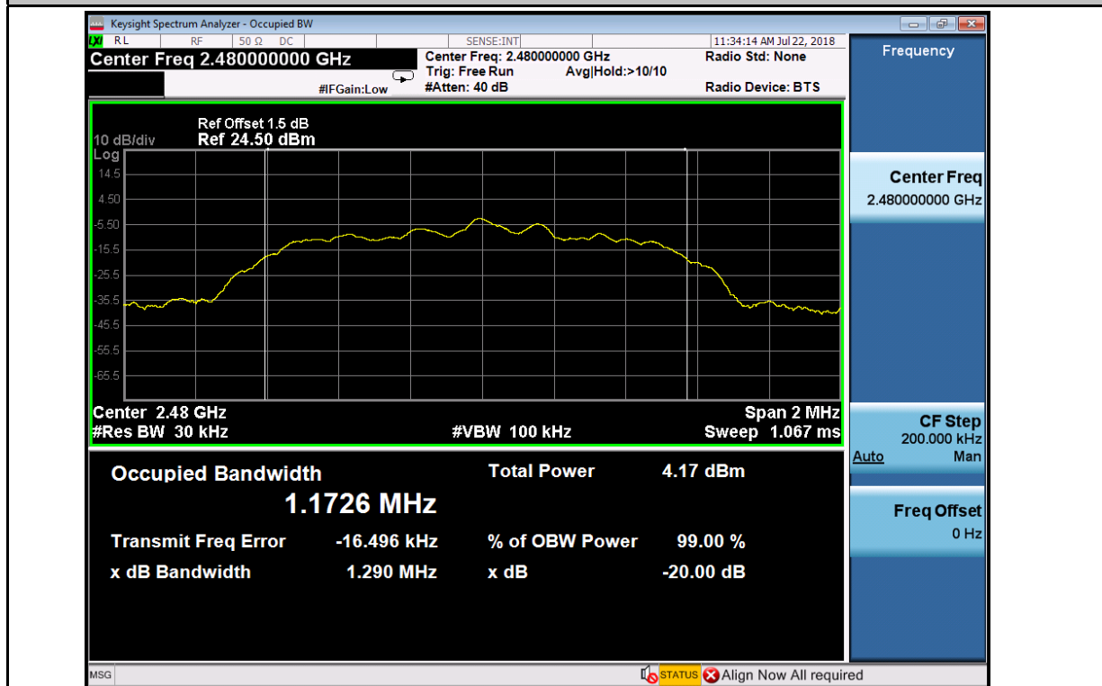
20 dB Bandwidth_2DH5_2480
