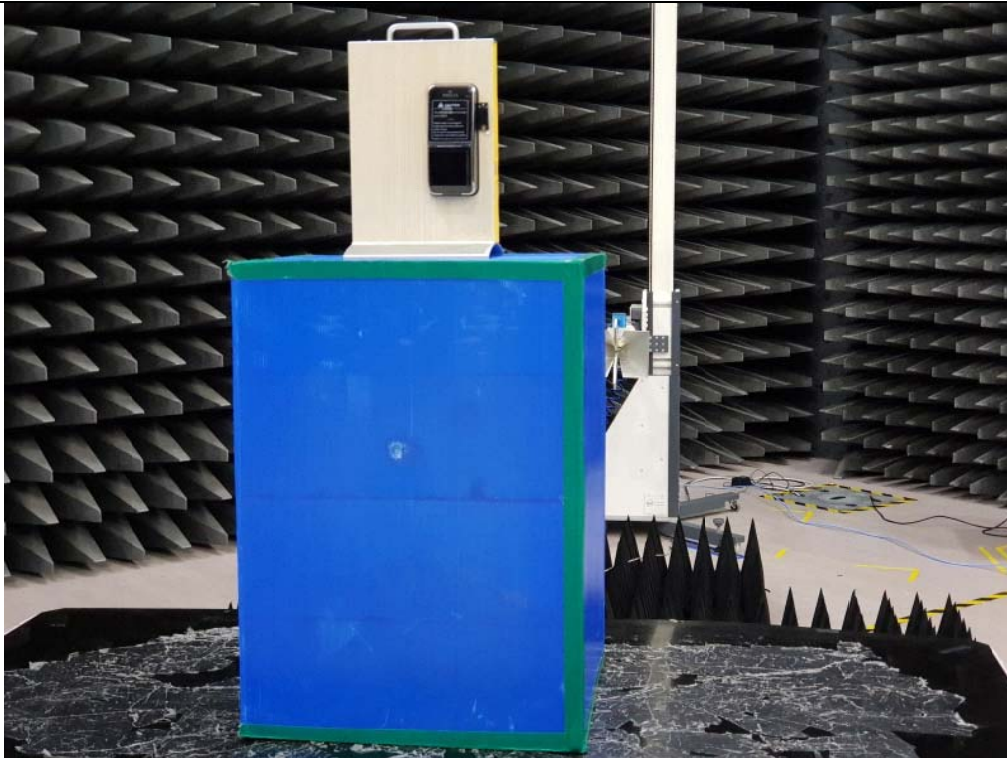
1 GHz – 10 GHz
