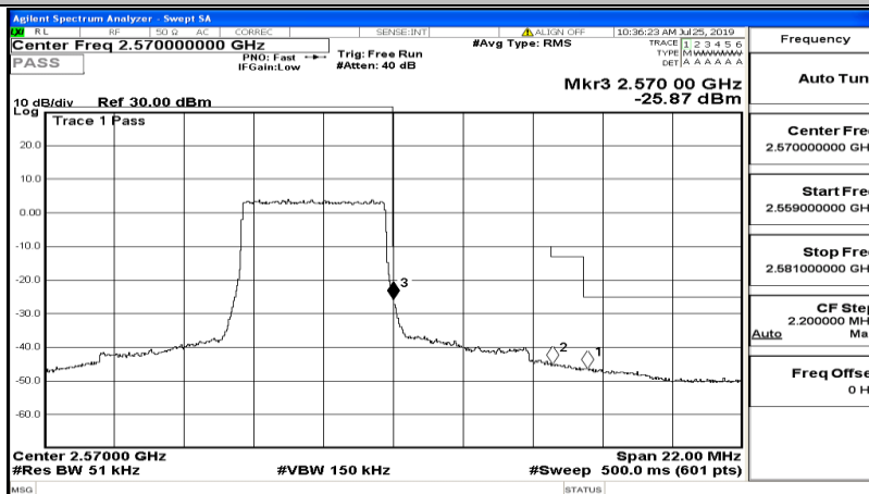
Band Edge Test Graph(s) (Channel Bandwidth: 5 MHz)_HCH_QPSK
