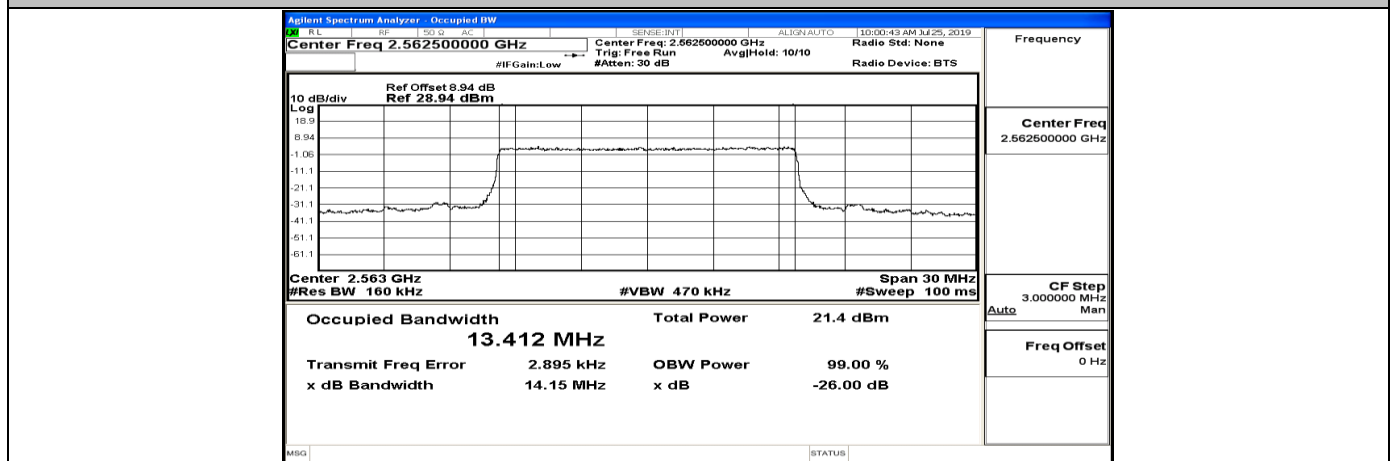
EBW &amp; OBW Test Graph(s) (Channel Bandwidth:15 MHz)_HCH_QPSK
