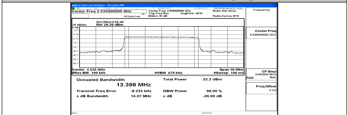
EBW &amp; OBW Test Graph(s) (Channel Bandwidth:15 MHz)_MCH_QPSK
