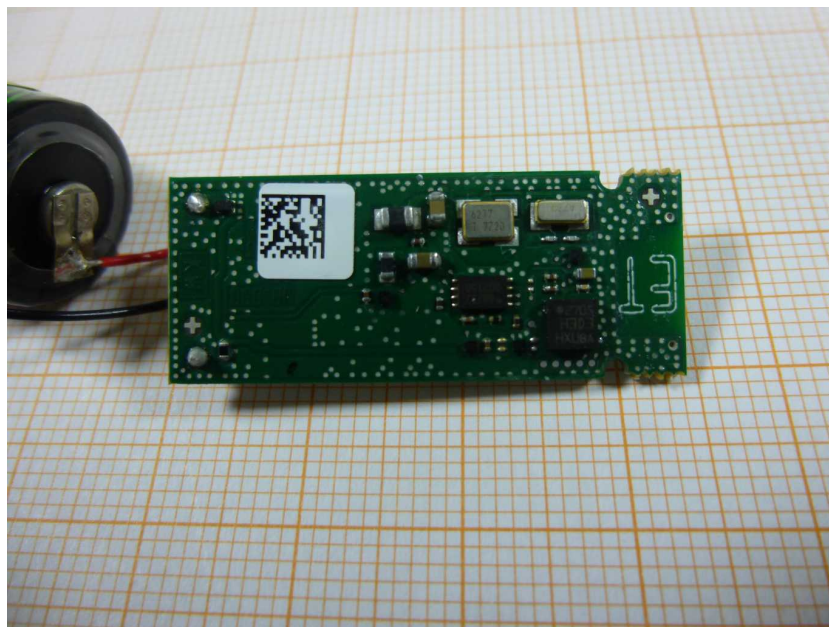
Photo 2: PCB back side view
