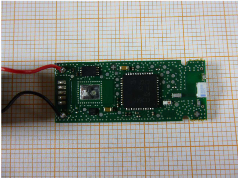
Photo 3: PCB front side view
