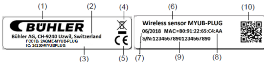
Fig. 4.1 Nameplate of MYUB-PLUG
