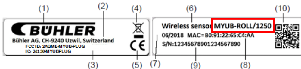
Fig. 4.2 Nameplate of MYUB-ROLL
