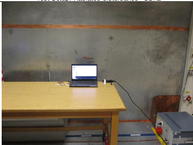
Test Setup: Conducted Emission on AC Power Line
