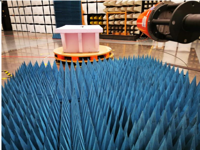
Test Setup: Radiated disturbance >1GHz
