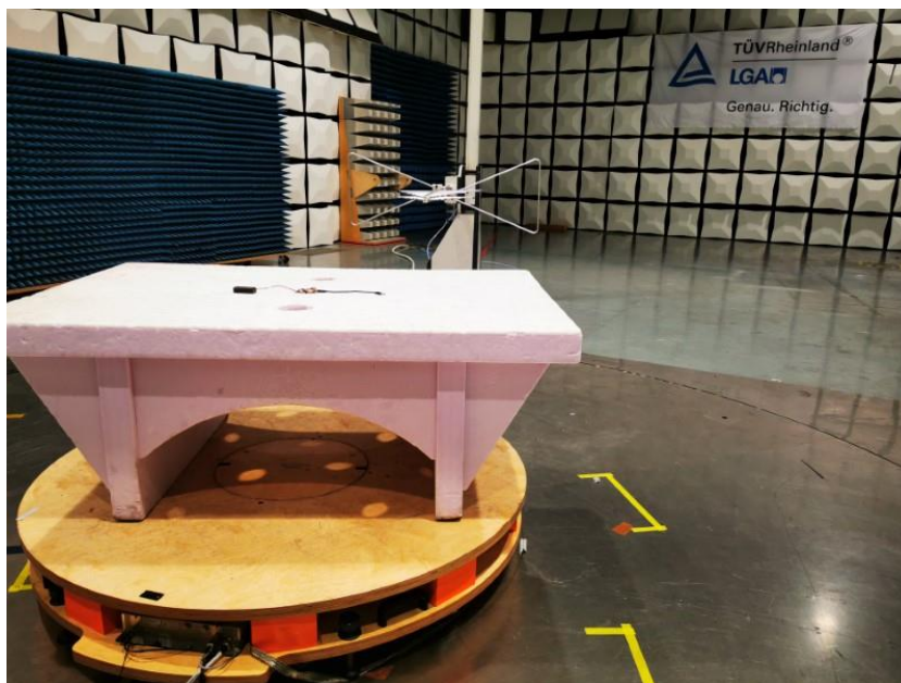
Test Setup: Radiated disturbance 30M-1GHz
