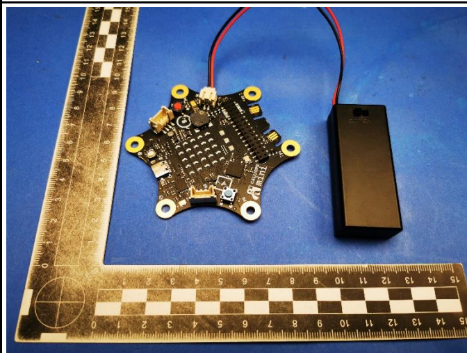
Picture 3 :EUT With Battery Holder
