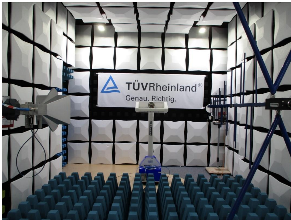
Test Setup: Radiated Measurements (1 GHz to 26 GHz)
