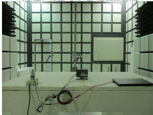
Part_15_247+RSS_247_WLAN_2.4G_Radiated_Setup
