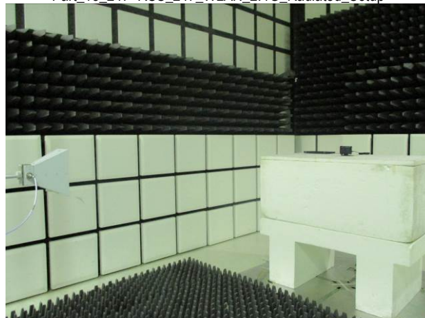
Part_15_247+RSS_247_WLAN_2.4G_Radiated_Setup
