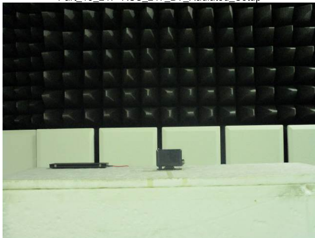
Part_15_247+RSS_247_BT_Radiated_Setup
