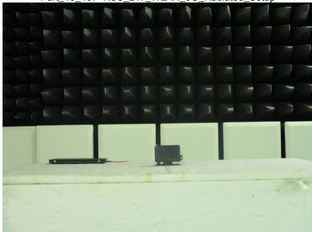
Part_15_407+RSS_247_WLAN_5G_Radiated_Setup
