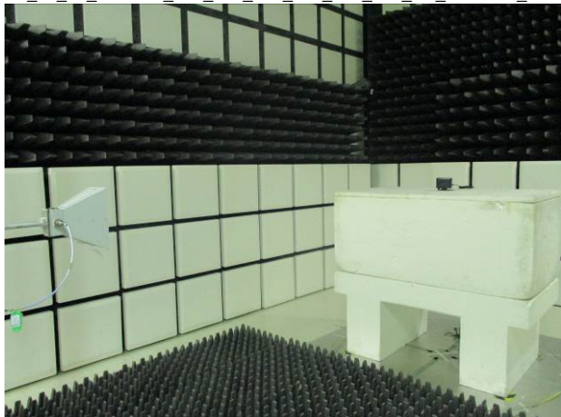
Part 22_24_27+RSS_130_132_133_139_140_199_4G_Radiated_Setup
