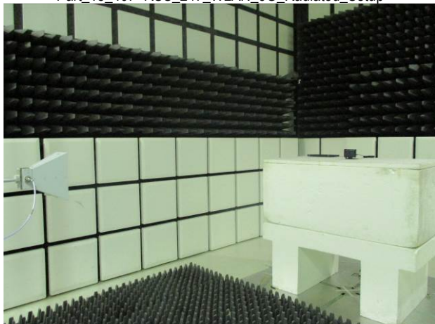
Part_15_407+RSS_247_WLAN_5G_Radiated_Setup
