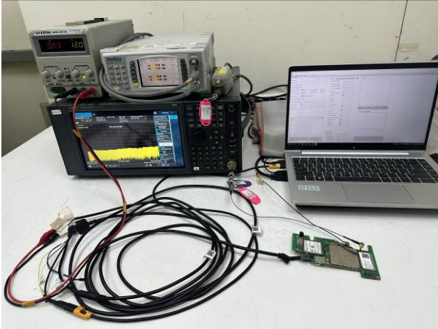
Part_15_247+RSS_247_WLAN_2.4G_Conducted_Setup
