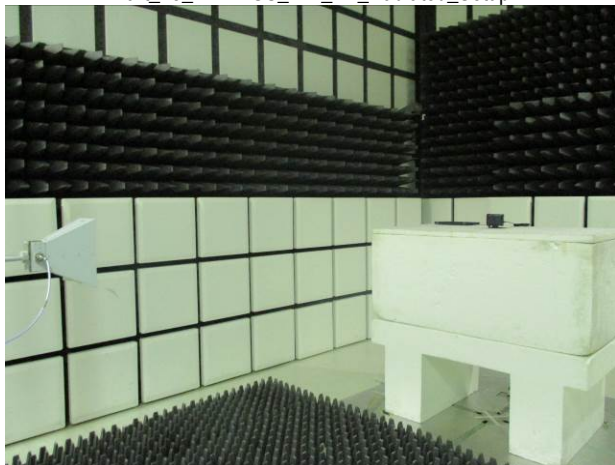
Part_15_247+RSS_247_BT_Radiated_Setup
