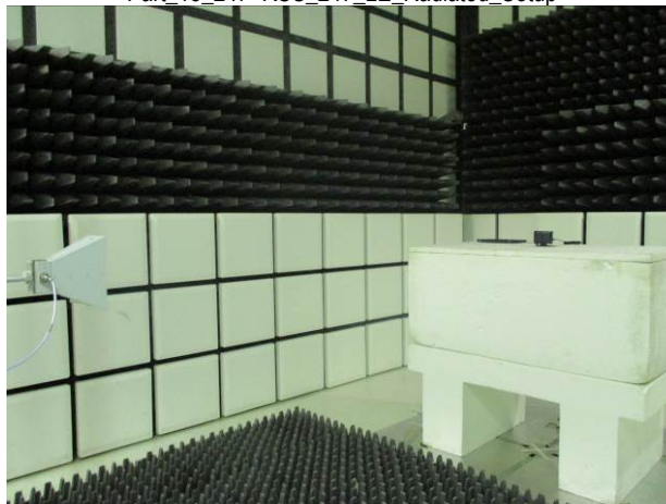
Part_15_247+RSS_247_LE_Radiated_Setup
