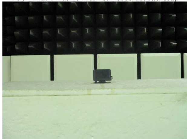
Part_22_24_27+RSS_132_133_139_2G&3G_Radiated_Setup
