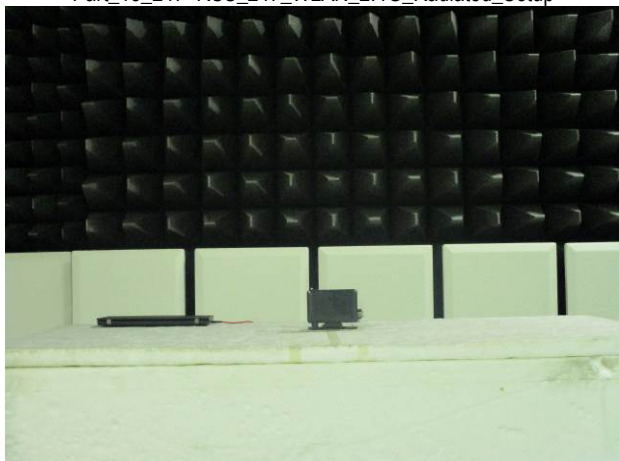
Part_15_247+RSS_247_WLAN_2.4G_Radiated_Setup
