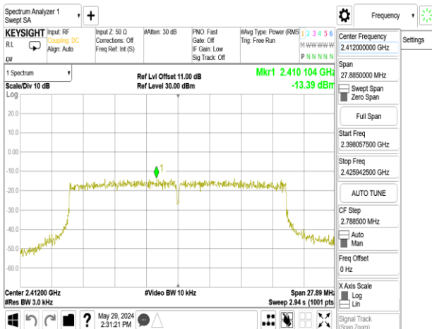
802.11ax_20MHz_Chain0_2412MHz_RU106_53
