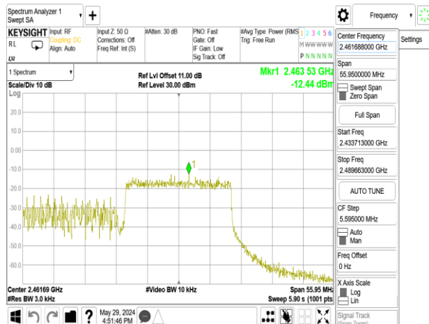
802.11ax_40MHz_Chain1_2452MHz_RU242_62
