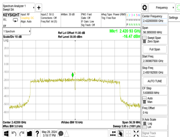
802.11ax_40MHz_Chain1_2422MHz
