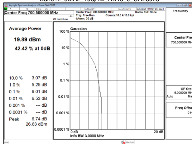
Band12_3MHz_16QAM_RB15_0_CH23095
