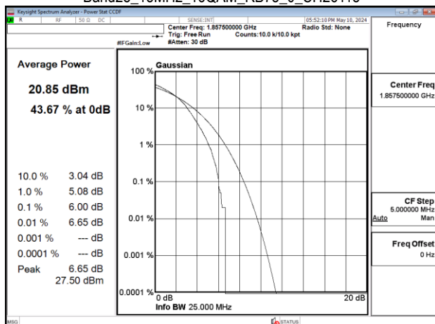
Band25_15MHz_16QAM_RB75_0_CH26115
