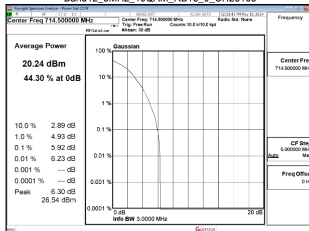
Band12_3MHz_16QAM_RB15_0_CH23165
