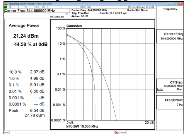
Band26_10MHz_16QAM_RB50_0_CH26990
