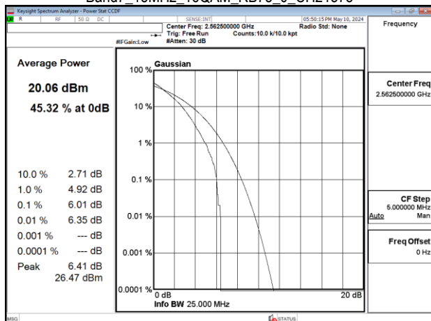
Band7_15MHz_16QAM_RB75_0_CH21375
