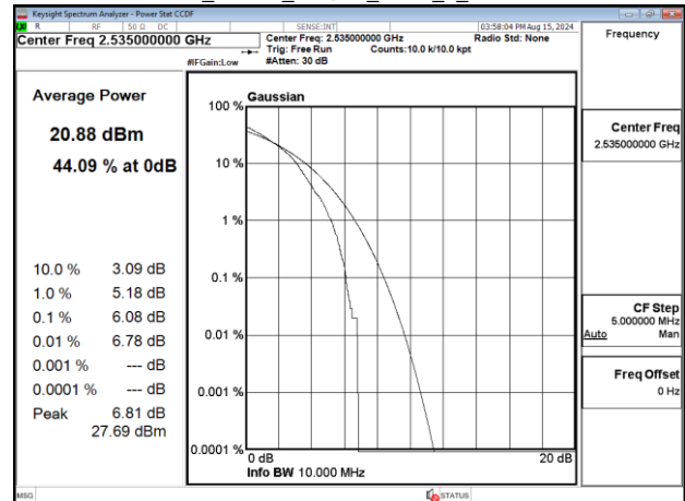
Band7_10MHz_16QAM_RB50_0_CH21400
