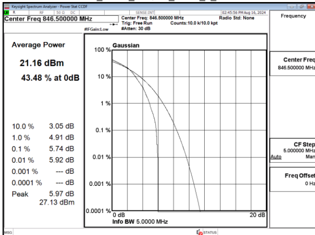
Band26_5MHz_16QAM_RB25_0_CH27015
