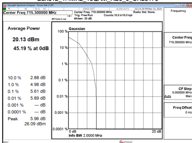
Band12_1.4MHz_16QAM_RB6_0_CH23173
