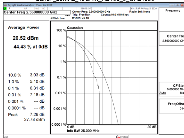
Band7_20MHz_16QAM_RB100_0_CH21350
