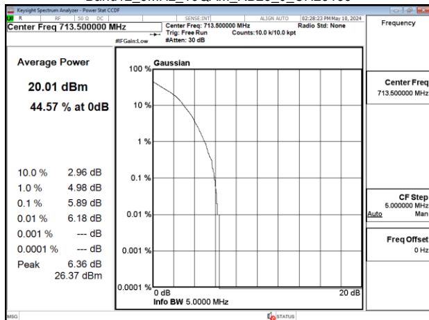
Band12_5MHz_16QAM_RB25_0_CH23155
