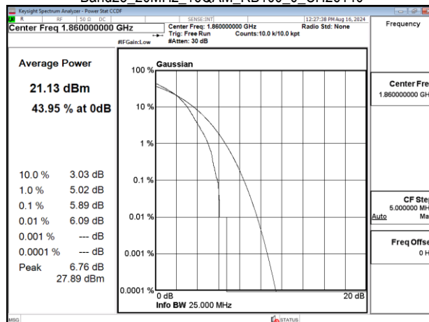
Band25_20MHz_16QAM_RB100_0_CH26140
