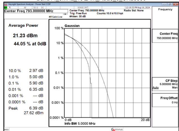
Band14_5MHz_16QAM_RB25_0_CH23330
