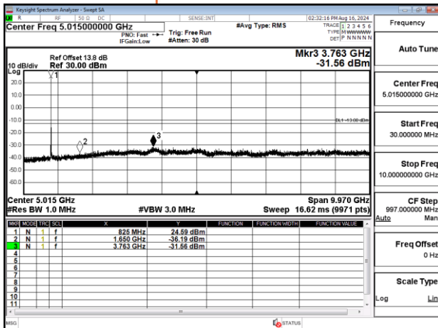
Band26_15MHz_QPSK_RB1_0_CH26915
