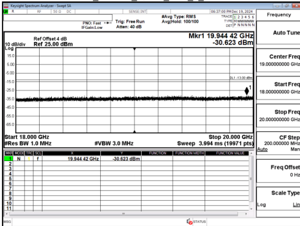
Band25_1.4MHz_QPSK_RB1_0_CH26683
