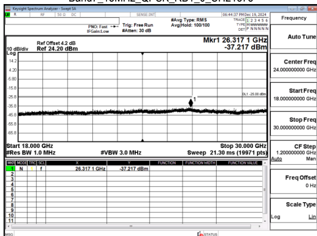
Band7_15MHz_QPSK_RB1_0_CH21375
