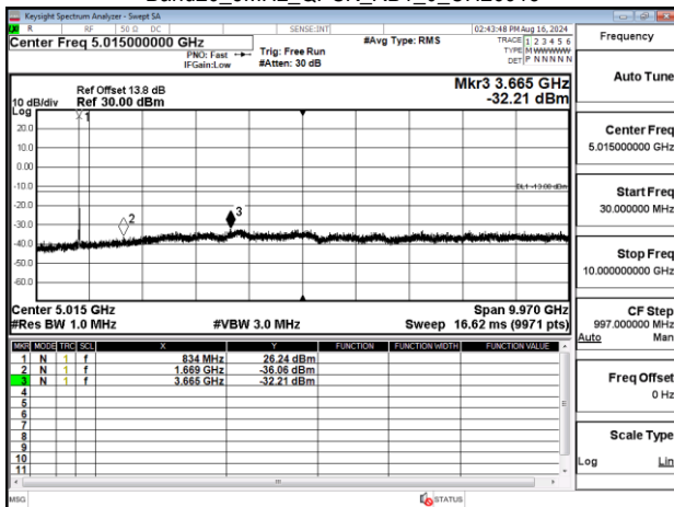
Band26_5MHz_QPSK_RB1_0_CH27015
