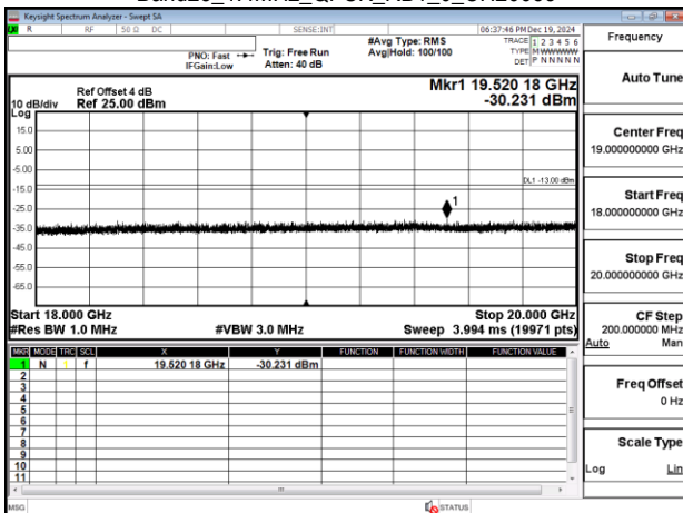
Band25_1.4MHz_QPSK_RB1_0_CH26683
