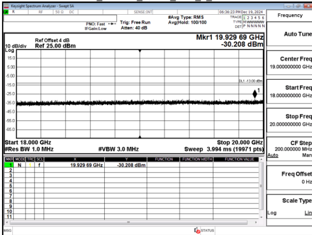
Band25_1.4MHz_QPSK_RB1_0_CH26365
