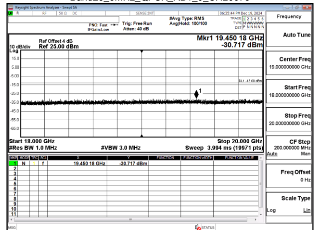
Band25_3MHz_QPSK_RB1_0_CH26675
