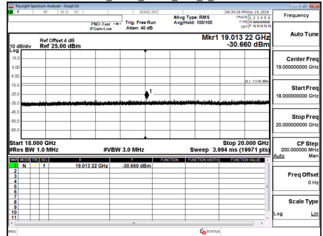
Band25_3MHz_QPSK_RB1_0_CH26365
