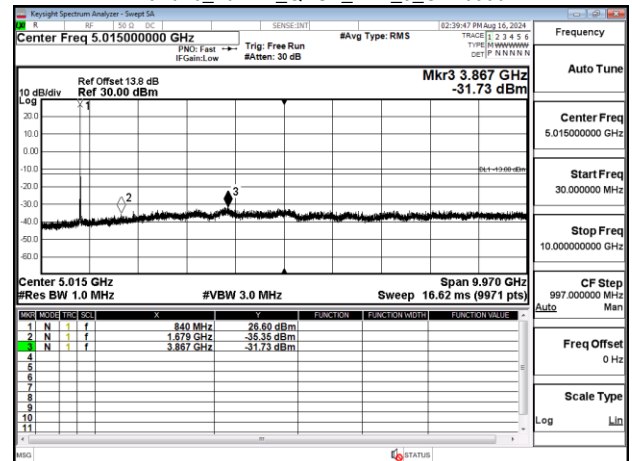
Band26_10MHz_QPSK_RB1_0_CH26990
