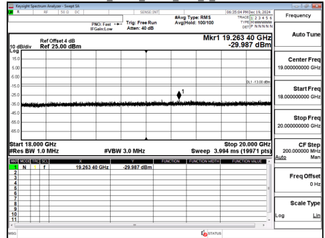
Band25_3MHz_QPSK_RB1_0_CH26675
