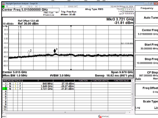
Band26_5MHz_QPSK_RB1_0_CH27015
